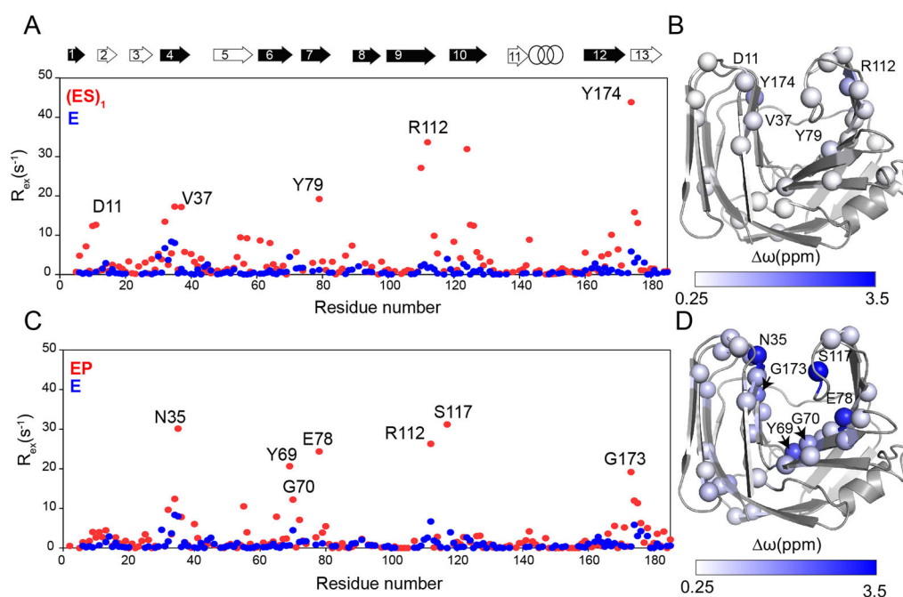
Figure 3. Non-covalent interactions enhance BCX millisecond time scale dynamics in the (\text{ES})_1 and EP states. A,C) Overlay of the R_{\text{ex}} values of (\text{ES})_1 (A) or EP (C) (red dots) and E states (blue dots) plotted versus the residue number. Several residues that show a prominent difference in R_{\text{ex}} are labeled. The secondary structure elements of BCX are represented by black arrows for \beta -strands of sheet A and in white ones for sheet B and the \alpha -helix in rings. The „thumb“ loop connects \beta -strands 9 and 10. B,D) Amide nitrogen atoms used in the RD global fit for (\text{ES})_1 (B) and EP (D) are shown in spheres on the BCX crystal structure (PDB ID: 2bvj) colored by their \Delta\omega between the ground and excited states, using a white/blue gradient. The \Delta\omega were derived from a global two-state fit to the dispersion curves.
