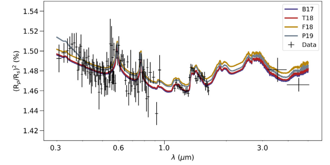
Figure 6. As Fig. 5 but for HD 209458b, for models including a fractional cloud parameter.
