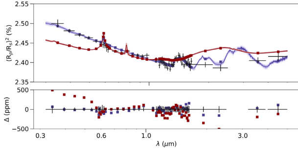
Figure 4. Spectral fits to the HD 189733b data (red) with the T18 model with a restricted temperature prior (dark red) and a broad prior (purple). Spectra are generated using the median values of the posterior distributions. The fit is generally poor for the restricted prior case as the relatively inflexible cloud parametrization does not allow the short wavelength slope to be matched. Shaded regions on the spectrum plot indicate the 2\sigma envelope for each case.
