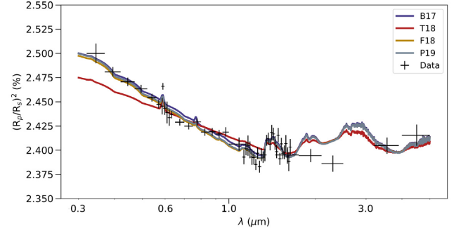
Figure 5. Spectral fits to the HD 189733b data for all models, for the restricted temperature case without fractional cloud. The model spectra are calculated using the median parameter values.
