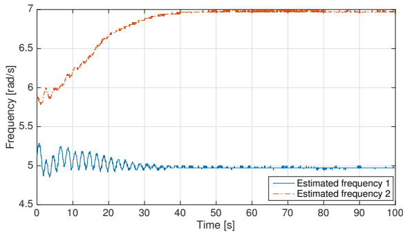
Fig. 13. Real-time frequency detection of a signal made up of two sinusoids by the proposed method
