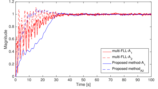
Fig. 5. Time-behavior of the estimated amplitudes by using the proposed method (blue) compared to the estimates by the method [22] (red).
