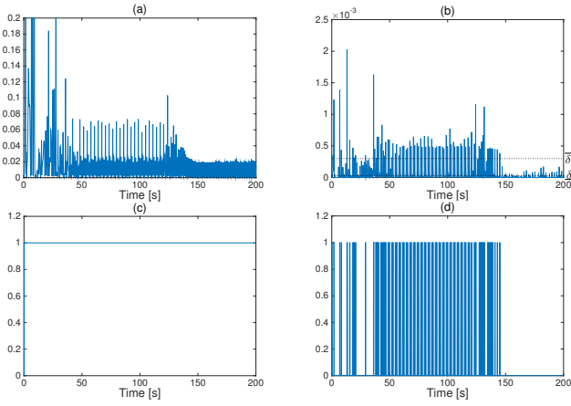
Fig. 7. (a) Excitation level \lambda_1(\Phi(\Xi(t))) ; (b) Excitation level \lambda_2(\Phi(\Xi(t))) ; (c) Switching signal \psi_1(t) ; (d) Switching signal \psi_2(t) .
