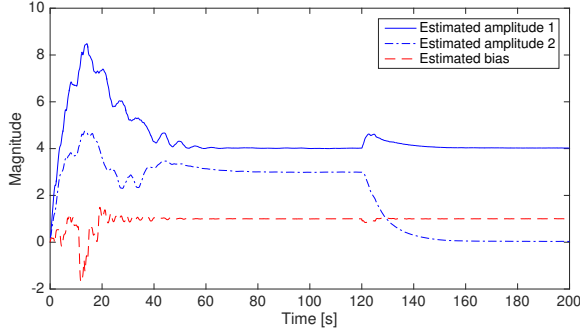
Fig. 9. Time-behavior of the estimated amplitudes (blue) and the estimated bias (red) by using the proposed method.
