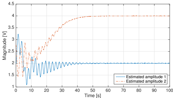
Fig. 14. Real-time amplitude detection of a single with two frequency contents by using the proposed method.
