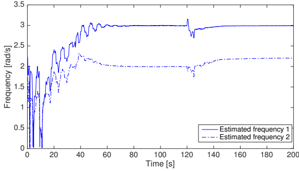
Fig. 8. Time-behavior of the estimated frequencies by using the proposed method.
