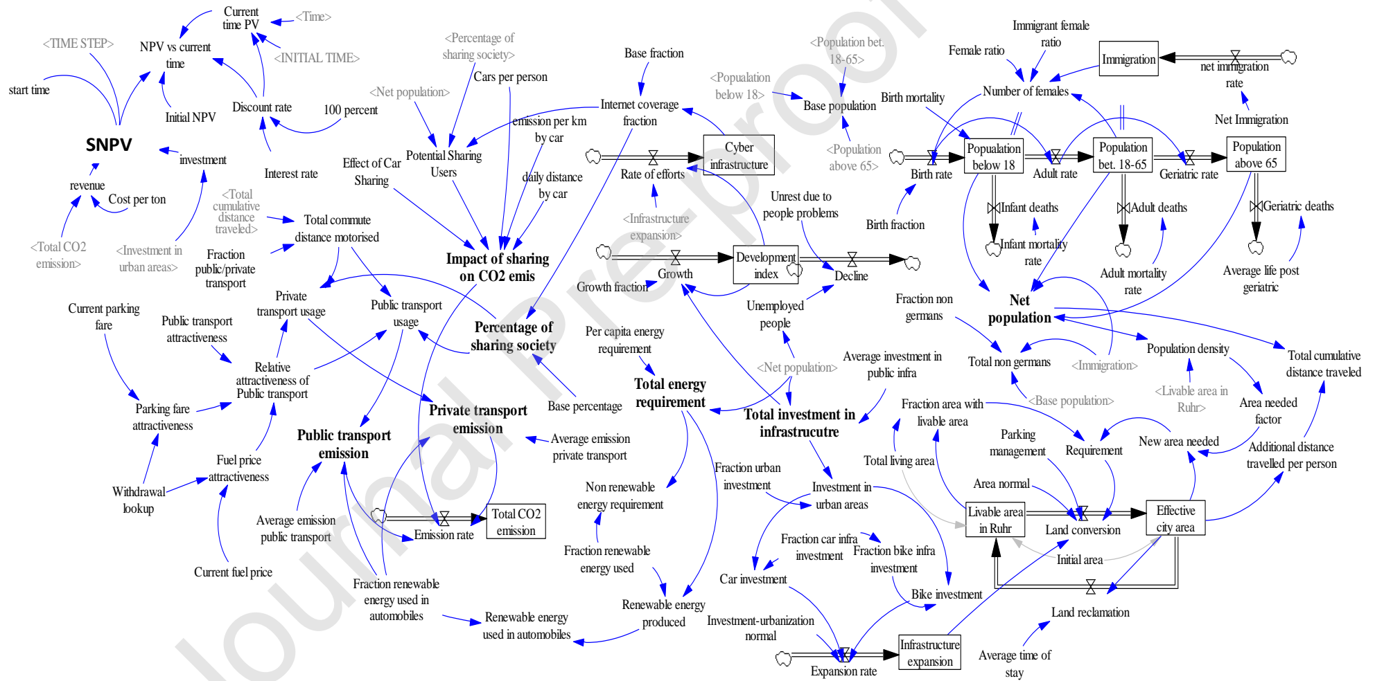
Figure 3: System dynamics simulation model of sustainable urban mobility turnover in the case of the Rhine-Ruhr metropolitan area
