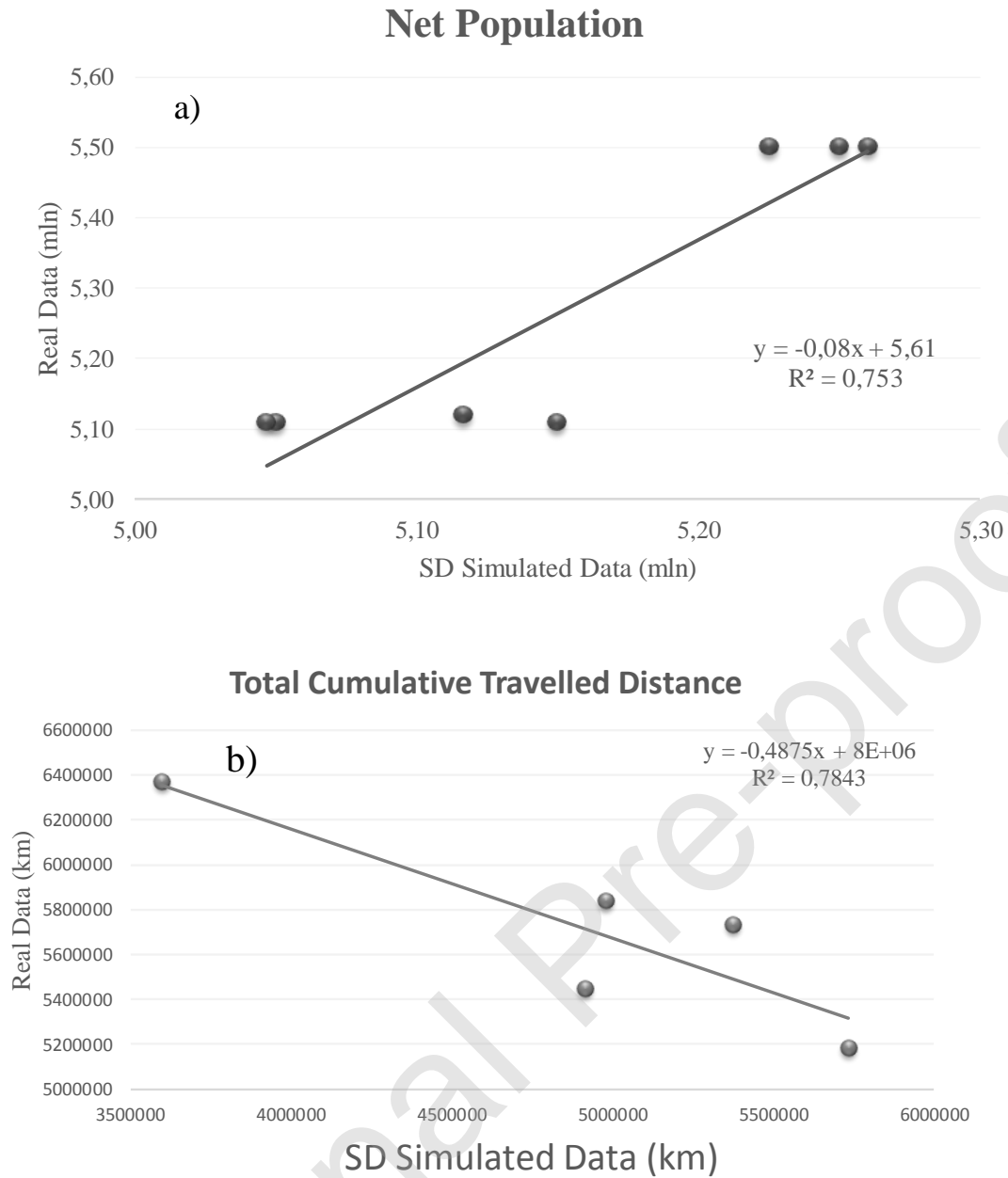
Figure A.-1: SD Model Validation for the output parameters a) Net Population and b) Total Cumulative Travelled Distance with the real data within the period of 2012-2018.
