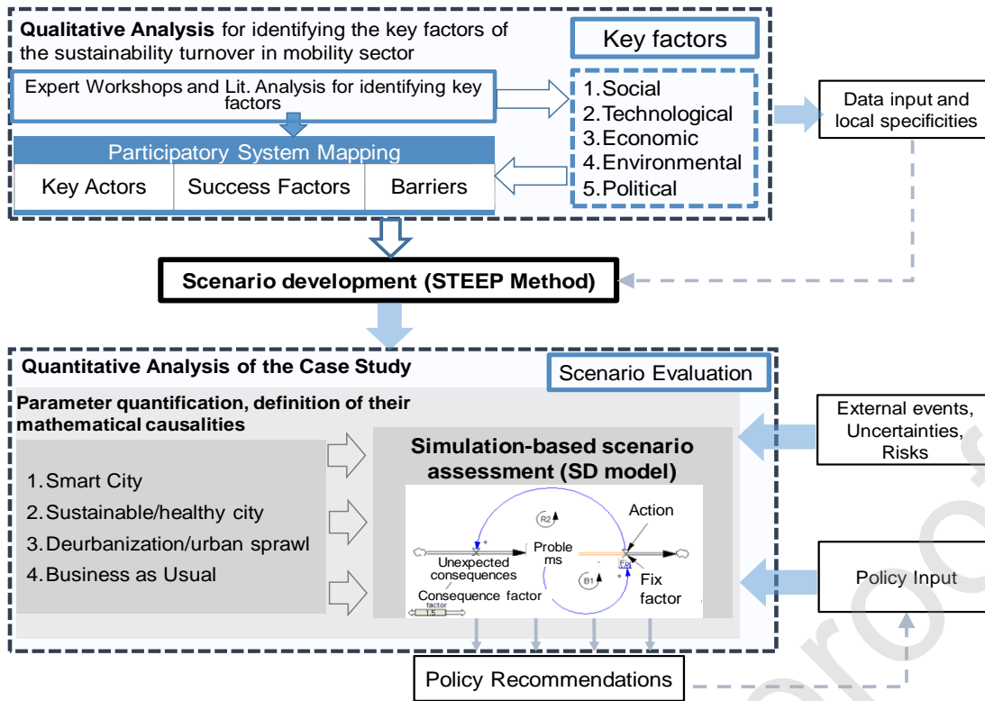
Figure 1: Simulation-based scenario assessment framework developed in this paper
