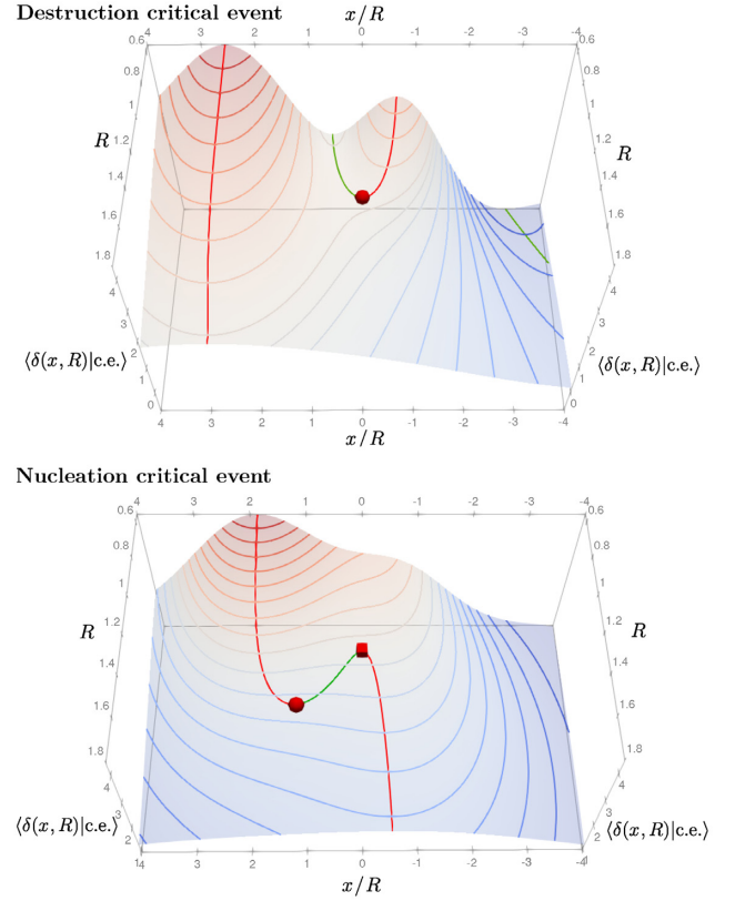
Figure 5. 2D slice, in the (x, R) plane, of the conditional mean density in the 3 + 1 D position–smoothing space, under the constraint of a destruction critical event (red sphere, top panel) and a nucleation critical event (red box, bottom panel) at R = 1 , x = 0 . The slice position is chosen to contain the events. Green lines show filament-type saddle points at each R and red lines show peaks. Density isocontours are represented as coloured lines (from red, high density to blue, low density). The top panel is reminiscent of Fig. 1, since 3D merger events closely resemble 1D merger events along filaments, while the bottom panel is unique to dimensions larger than one for Gaussian smoothing. An interactive version can be found in the online supplemental material and online. While nucleation events such as that shown on the bottom panel can occur, they statistically seem to remain short-lived and are less frequent than destruction ones.
