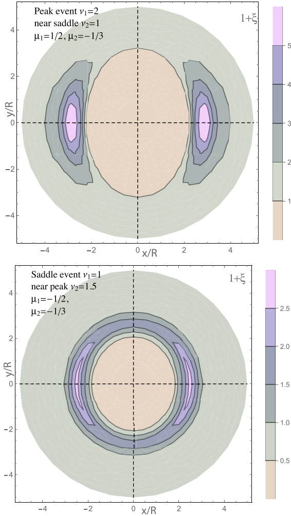
Figure 10. Theoretical prediction for the conditional excess probability, 1 + \xi , of peak merger events in the frame of a 2D critical point at the origin as labelled. The critical point defines a local exclusion zone whose geometry is set by its fixed eigenvalues. For simplicity, we have chosen R_c = R , while the underlying power spectrum index is -1 . See Fig. 17 for measured 3D counterparts.
