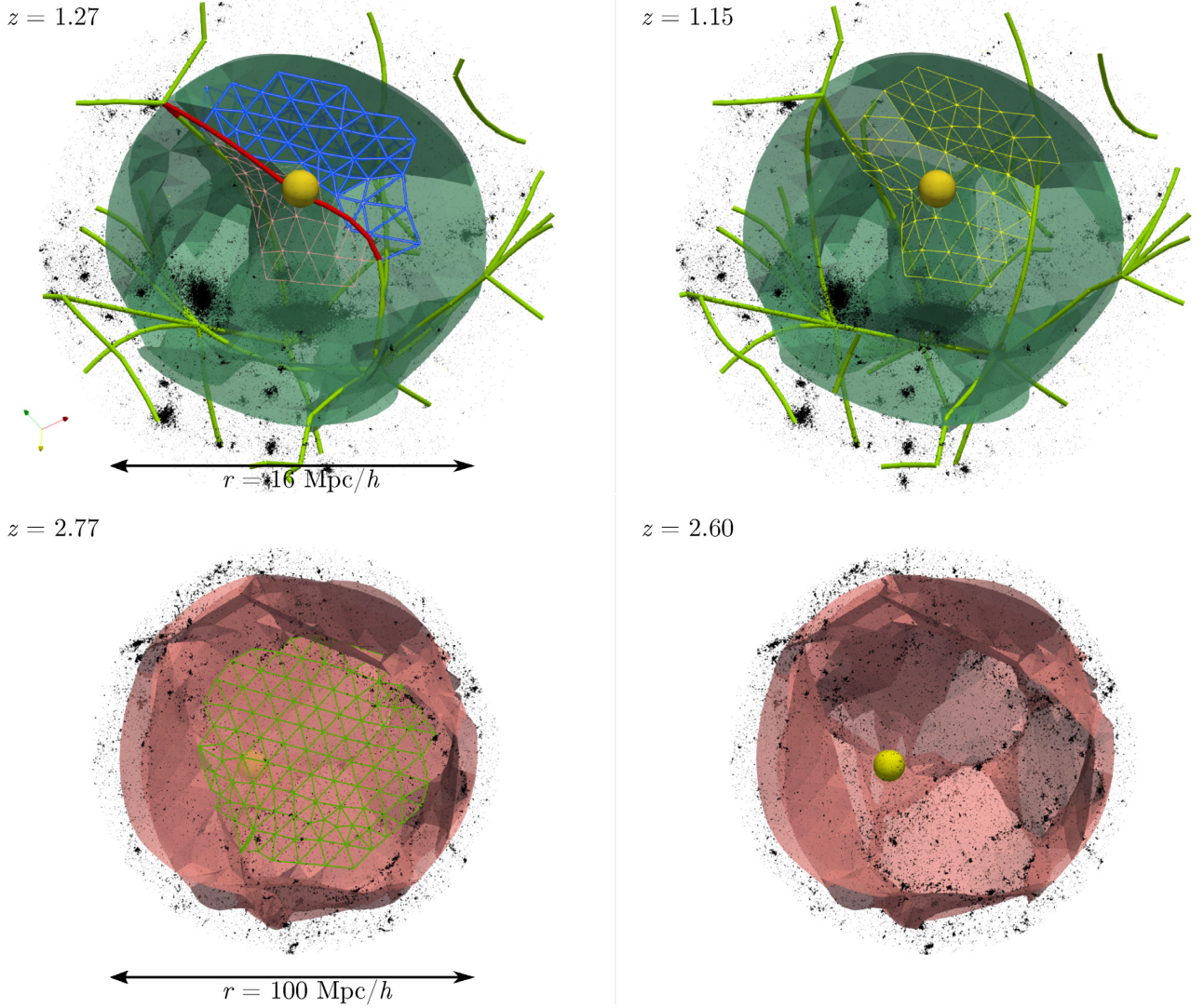
Figure 19. Top panels: two consecutive snapshots in a 100 \text{ Mpc } h^{-1} simulation showing an \mathcal{F} critical event (yellow ball) that encodes the disappearance of a filament (highlighted in red) separating two walls (red and blue wireframes). After the event, only one wall has survived (yellow wireframe). Bottom panels: two consecutive snapshots in a 500 \text{ Mpc } h^{-1} simulation showing a \mathcal{W} critical event (yellow ball) that encodes the merger of two voids separated by a wall (green wireframe). After the event, only one void subsists and the wall has disappeared. Individual DM particles are shown as black dots. The skeleton (green lines) and the walls (green and red surfaces) have been extracted using DISPERSE. Both critical events can be related to merger event in the evolved Universe.
