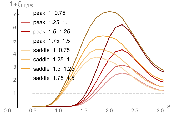
Figure 9. Same as Fig. 8 for the two-point correlation of events in 2D fields with scale-invariant power spectrum of index n_s = -1 . Next, filament mergers will occur before next peak mergers. The rarer the event, the more delayed, and the higher the clustering amplitude.
