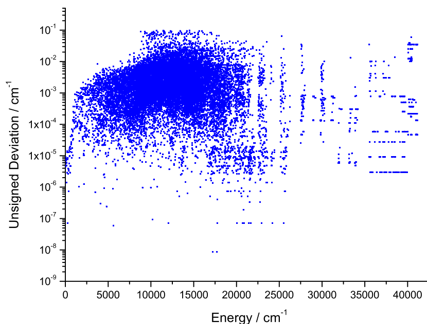
FIG. 4. Unsigned deviations of the Part III 3 energy levels from their W2020 counterparts. The states (both Part III and W2020) that could not be matched within 0.1 cm -1 are listed in the supplementary material .
