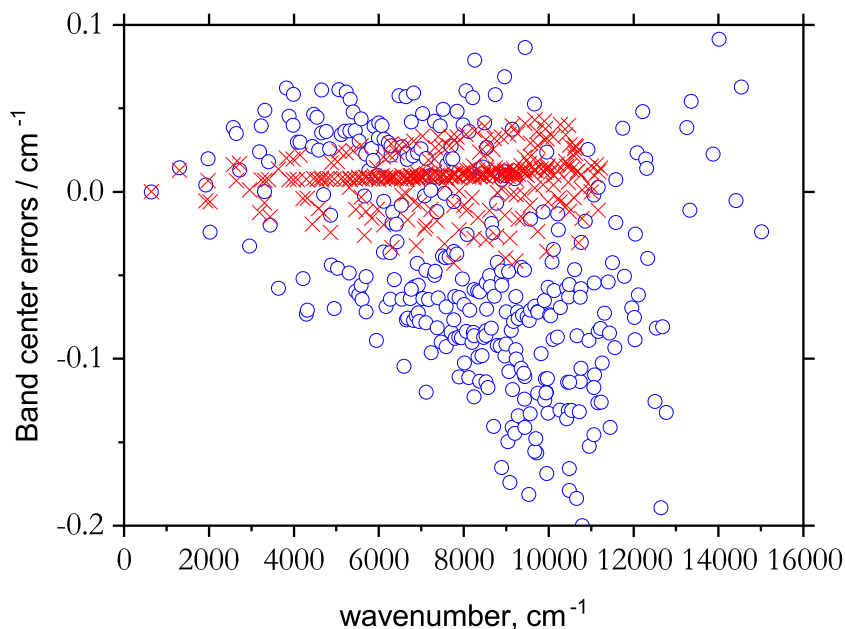
Figure 1. Blue circles: Average ro-vibrational errors for 337 vibrational ( J = 0 ) states from HITRAN estimated as CO 2 \tilde{E}_\lambda^H - \tilde{E}_\lambda^T (HITRAN–TROVE) term values for J \leq 40 , which were used as band centre corrections (see the text). Red crosses: Average residuals for the ro-vibrational CO 2 term values (for J \leq 40 ) between TROVE (before the band centre correction) and calculations from Zak et al. (2016) using DVR3D and the same PES Ames-2016 for 294 vibrational states.
