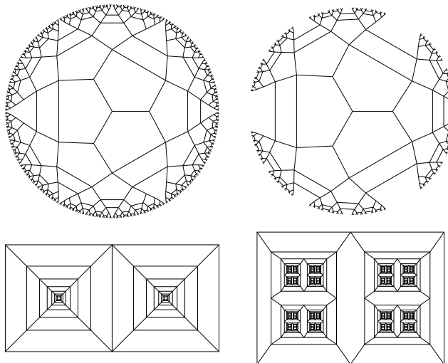
FIGURE 6. Four examples of self-accumulation-free pointed embeddings of 3-connected graphs, demonstrating some of the different possibilities for the set of endpoints and the boundaries of faces.
