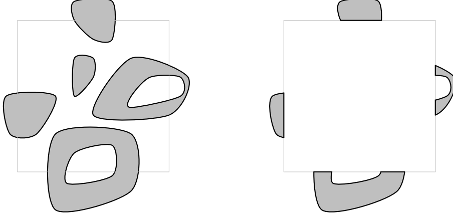
FIGURE 5. Simple contours intersecting the square \overline{\Delta_0} colored with two colors: 1 (white) and 2 (gray). After flipping all sites in \Delta_0 to the color 1, no contour is intersecting \Delta_0 and no triple point was created. The same would be true when flipping all sites in \Delta_0 to the color 2.
