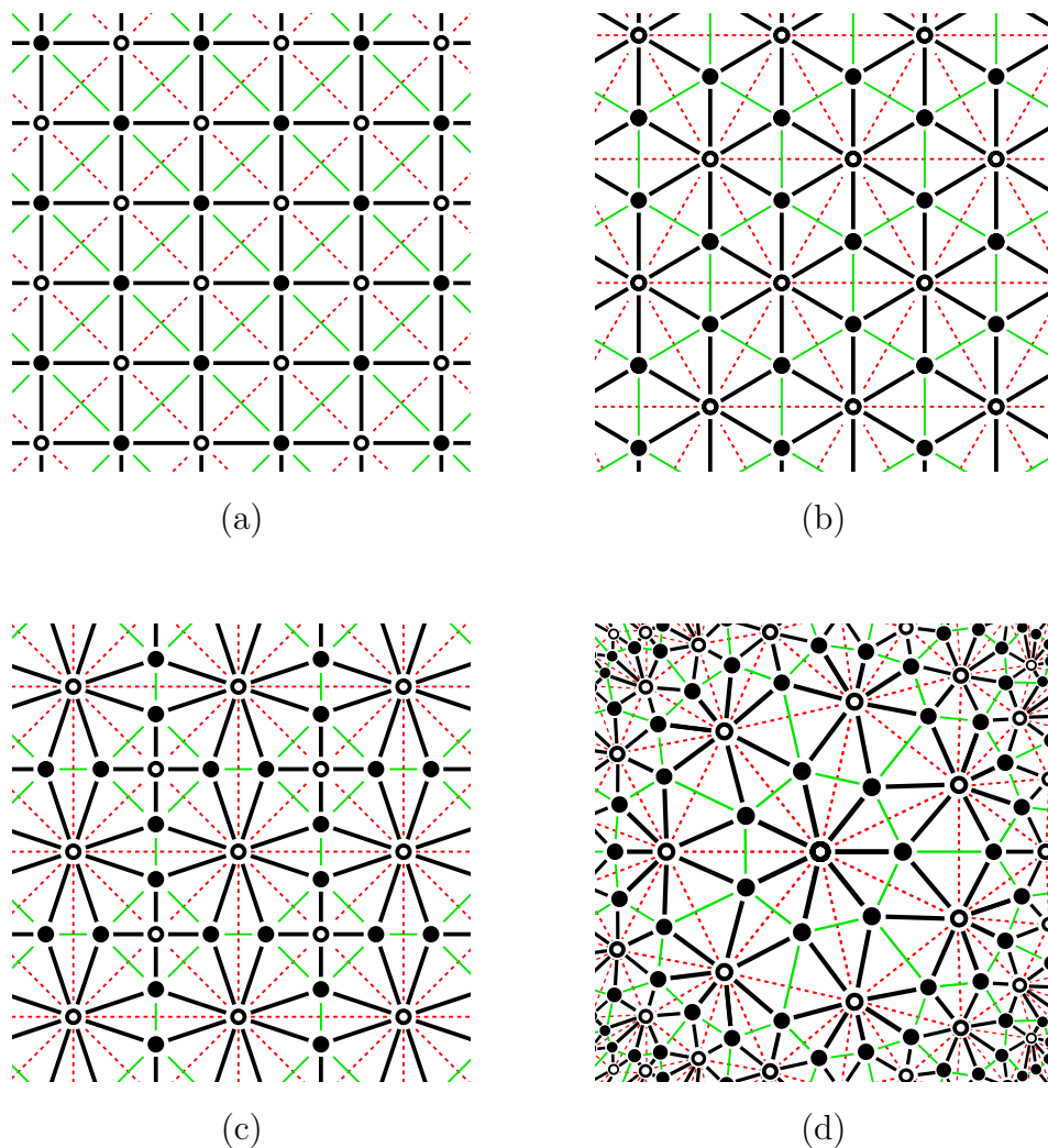
FIGURE 1. Four quasi-transitive quadrangulations with their sublattices G_0 (open circles joined by dashed red edges) and G_1 (filled circles joined by solid green edges). In these examples, the sublattice G_0 is (a) the square lattice, (b) the triangular lattice, (c) the union-jack lattice, and (d) the hyperbolic lattice with Schläfli symbol \{3, 7\} . Note that in (b)–(d), G_0 is a triangulation. In (a) and (b), the quadrangulations G are, respectively, the square lattice and the diced lattice.
