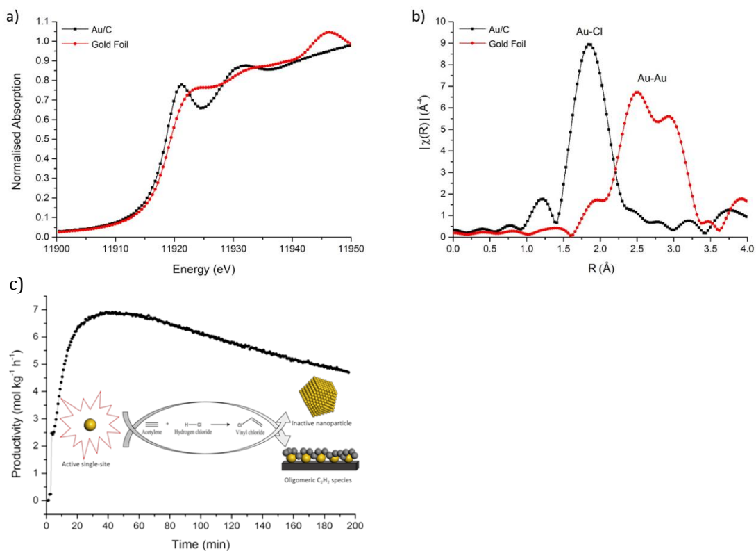
Figure 2. Au L_3 -edge a) normalised XANES and b) Fourier transform of k^3 -weighted \chi EXAFS spectra of the Au/C catalyst (black squares) and a gold foil reference material (red circle), c) Schematic representation of the deactivation pathways of single-site Au/C catalyst during the acetylene hydrochlorination reaction
