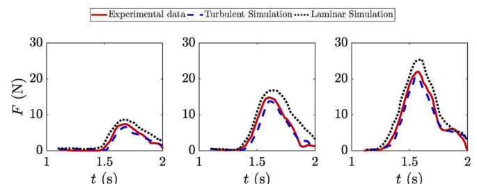
Fig. 9. Time histories of the impact force acting on the step.
