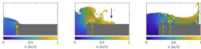
Fig. 15. Samples of the velocity plot of shipping water washing the step (grey box). The left panel shows the early stage of the washing as water reaches the step. The middle panel shows a point in time when the water has travelled some length over the step. The right panel shows a point in time at which water has reached the right wall of the tank. All simulations correspond to Case 5 and Tank 1.
