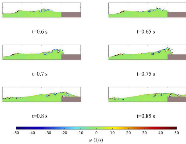
Fig. 10. Shipping water washing the deck of a step. Temporal snapshots present the vorticity field ( \omega ) and correspond to Case 3 in Tank 1. The step is depicted by the grey box.
