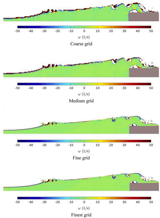
Fig. 4. Vorticity ( \omega ) for Case 4 with different grid sizes. (Dam-break in Tank 1).
