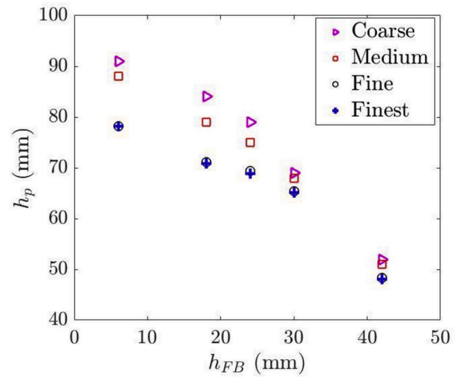
Fig. 3. Mesh convergence study showing maximum water surface elevation ( h_p ) versus freeboard ( h_{FB} ) for the shipping water at a distance of 0.0130L from the front edge of the step. (Dam-break in Tank 1).
