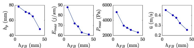
Fig. 16. Maximum values of (from left to right): water height ( h_p ), energy flux ( E_{max} ), hydrodynamic pressure ( P_{max} ) and mean horizontal velocity ( \bar{u} , at time t = 0.02 s after water reaches the front edge of the step) as a function of freeboard ( h_{FB} ). (All results correspond to Tank 1).
