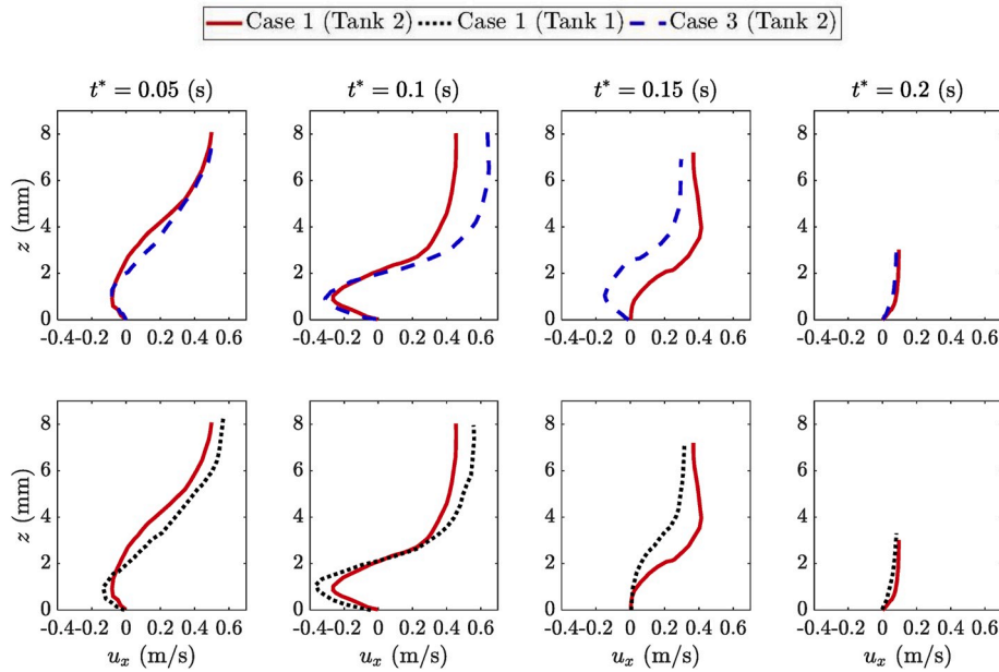
Fig. 14. Profile of the horizontal velocity of the shipping water at the front edge of the step at different times. The upper panels show a comparison between the velocity profiles of Cases 1 and 3 (Tank 2). The lower panels show the comparison between the velocity profiles for Case 1 in Tanks 1 and 2.
