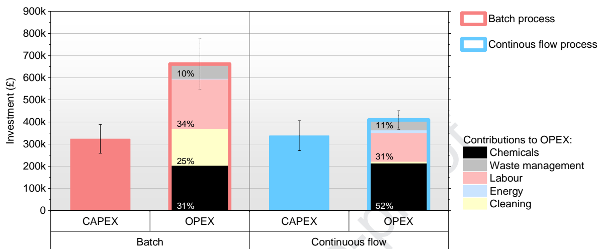
Figure 9 –Comparison of operating expenses (OPEX) with relative contributions, and capital expenses (CAPEX) for batch and continuous flow process
