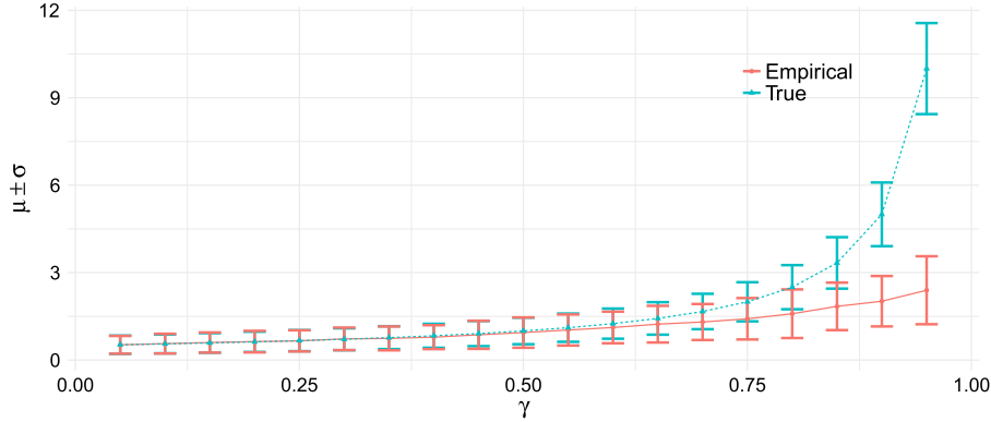
FIG 2. Empirical vs asymptotic mean of nMMD(\hat{F}_n, F_0) for different values of \gamma < 1 . For each value of the mean \mu and \hat{\mu} , we plot the intervals [\mu - \sigma, \mu + \sigma] and [\hat{\mu} - \hat{\sigma}, \hat{\mu} + \hat{\sigma}] , where \hat{\sigma}^2 and \sigma^2 denote the empirical and asymptotic variance respectively. We use a fixed sample size n = 3000 .
