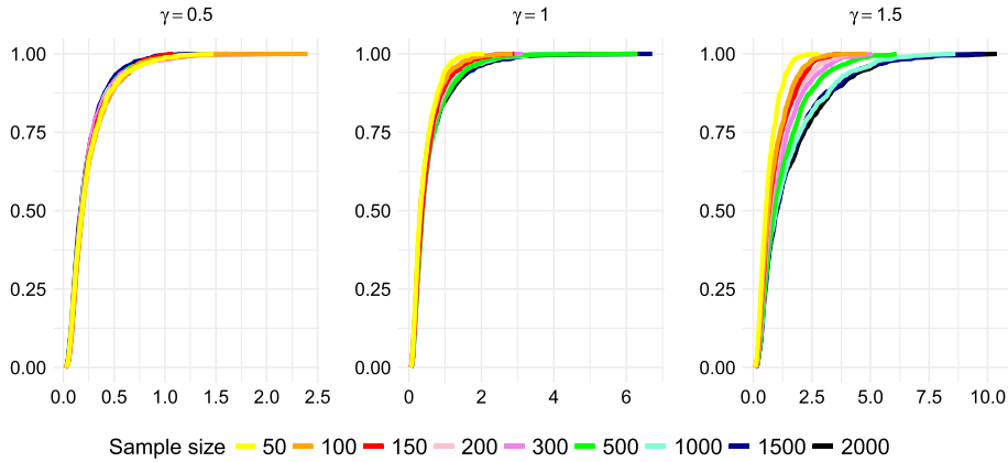
FIG 1. Empirical distribution functions of n\theta(\widehat{F}_n) for different sample sizes and values of \gamma . Each empirical distribution was computed using 1000 independent realisations.
