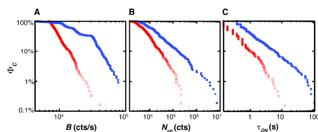
Figure 1. \Phi_C for B (A), N_{ph} (B) and \tau_{ON} (C) of MC single molecules embedded in PPMA thin films of 23 \pm 3 nm thickness detected over 68 nm diameter AuNPs (blue). Similar data collected in the absence of AuNPs (red) are also shown.
