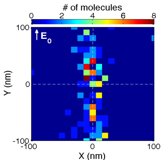
Figure 2. Super resolution localization of MC single molecules detected over a single AuNP (2D-histogram, 10 x 10 nm 2 bins). Their position is referred to the nearest AuNP in the image field. The histogram was constructed with all the MC molecules that displayed \tau_{ON} > 5 s (data from all the different film thicknesses). The laser polarization direction is along the y-axis.
