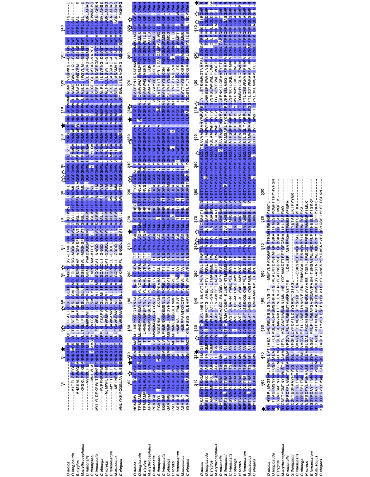
Figure 2. Sequence alignment of Cox1 proteins. White stars indicate conserved cysteines when at least one tunicate uses an AGR codon. Black stars indicate positions suggesting a different genetic code.
