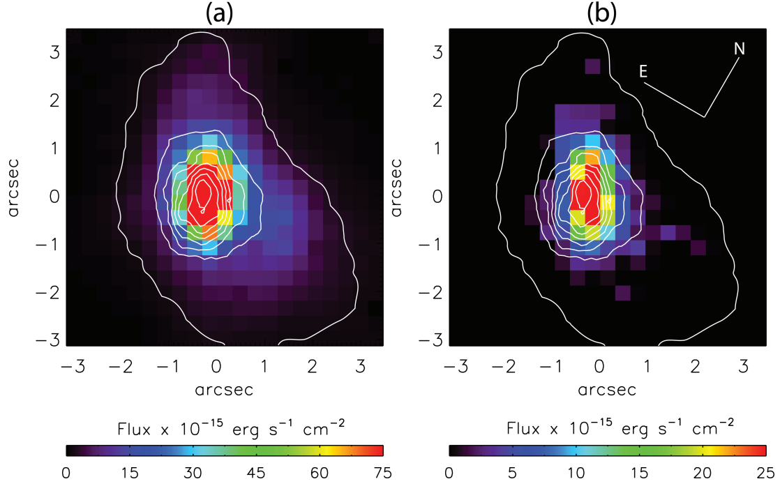
Figure 7. [O III] \lambda 5007 emission line maps of Mrk 996 showing the flux distribution per 0.33 \times 0.33 \text{ arcsec}^2 spaxel: (a) in the narrow C1 component; (b) in the broad C2 component. Overlaid are the H \alpha narrow component contours (white), as shown in Fig. 1.
