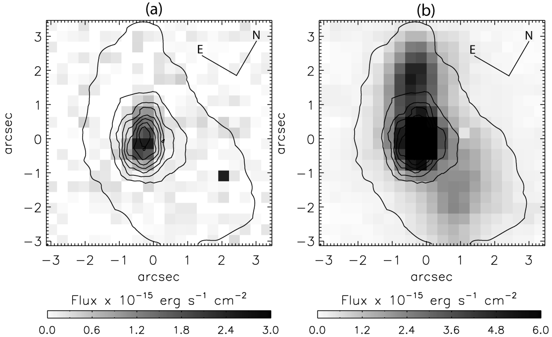
Figure 10. Flux distribution per 0.33 \times 0.33 \text{ arcsec}^2 spaxel of (a) [N II] \lambda 5755 for which only a broad component is detected and which is seen only within the core region; (b) [N II] \lambda 6584 , whose flux distribution peaks in the core and towards the north-east; a fainter peak is seen west of the core. Overlaid are the \text{H}\alpha narrow component contours as shown in Fig. 1.
