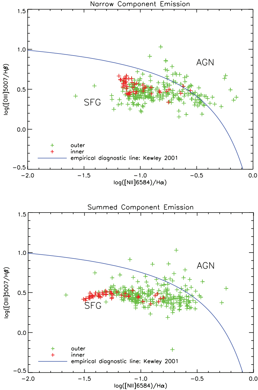
Figure 22. Emission line diagnostic diagram for Mrk 996. Each data point represents a spaxel in the ratioed dereddened flux maps corresponding to [\text{O III}] \lambda 5007/\text{H}\beta and [\text{N II}] \lambda 6584/\text{H}\alpha . The empirical diagnostic ‘maximum SB’ line from Kewley et al. (2001) is also shown, as are the positions of emission line ratios for SFG and AGN. The top panel represents narrow component emission line map ratios whereas the bottom panel shows ratios derived from the full emission line profile (i.e. narrow + broad component emission, where detected).
