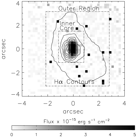
Figure 8. Flux distribution of [O III] \lambda 4363 per 0.33 \times 0.33 \text{ arcsec}^2 spaxel with H \alpha contours overlaid. The area over which \lambda 4363 is detected is used to define an ‘inner core’ region, with a surrounding ‘outer region’ covering the full extent of the H \alpha emission.
