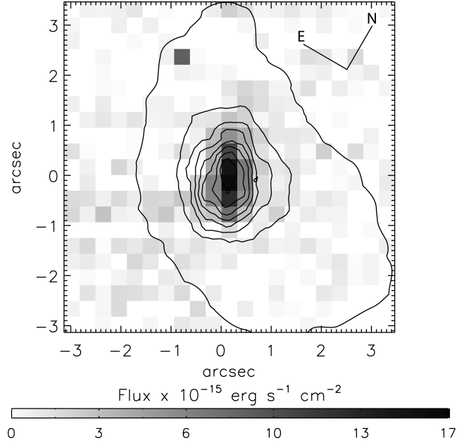
Figure 19. Emission map of the blue WR feature (created by integrating over the full emission feature and removing contaminant flux from [Fe III] \lambda 4658 ), showing the distribution of WR stars in the inner core region of Mrk 996. Overlaid are the \text{H}\alpha narrow component flux contours from Fig. 1.
