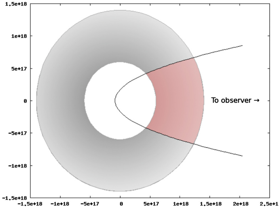
Figure 4. Schematic of the fraction of the CSM ejecta which will have been lit when light travel times are taken into consideration. For the example above, at 90 days, only about 5% would have been illuminated.
