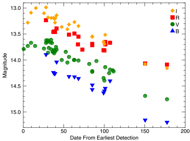
Figure 2. Optical light curve of SN 2010jl. Data are from AAVSO, Stoll et al. (2010), and new data presented in Table 2 in this paper.
