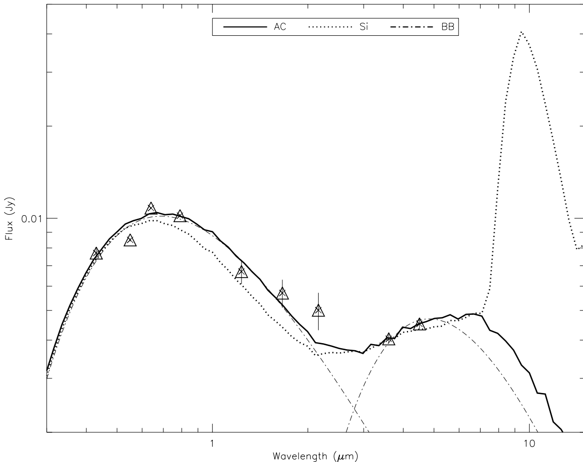
Figure 3. SED of SN 2010jl on \sim day 90. IR photometry is listed in Table 3, and optical photometry was obtained from the AAVSO, specifically contributor Etienne Morelle. Dash-dotted lines are the blackbody fits to the data. The solid line indicates the 100% amorphous carbon inclined at 60^\circ MOCASSIN torus model fit, the dotted line is the same except for the composition being 100% silicates. As the figure shows, without observations longward of 4.6 \mu\text{m} , we cannot accurately constrain the dust composition.
