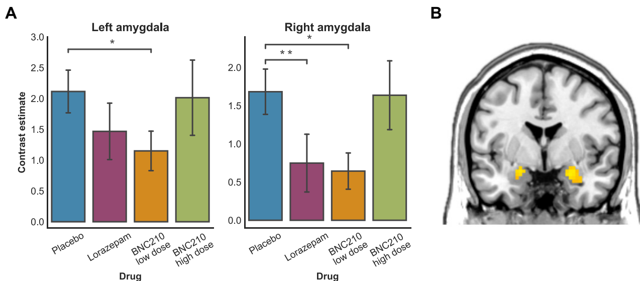
Figure 2. (A) Mean ( \pm SE) amygdala response to fearful faces for each drug condition. (B) Effect of BNC210 low dose on amygdala activity, thresholded at p < .05 uncorrected for illustration. * p < .05 , ** p < .01 .
