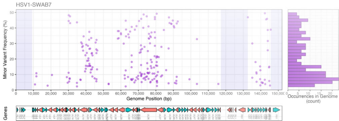
Figure 4. Frequency of HSV1-SWAB7 minor variants across the genome. Minor variant frequencies (estimated with a mean read depth of 3,354 \times ) show a mixed pattern of intra-host allelic diversity, with variants occurring at many different frequencies without clustering. This pattern suggests intense recombination between different virus types, possibly emerged from extensive intra-host evolution. Plots show frequency of variant alleles by genomic position (left) and frequency histogram (right, 2% intervals), with corresponding gene positions below. Shaded region indicates repeat regions with no mapped reads.
