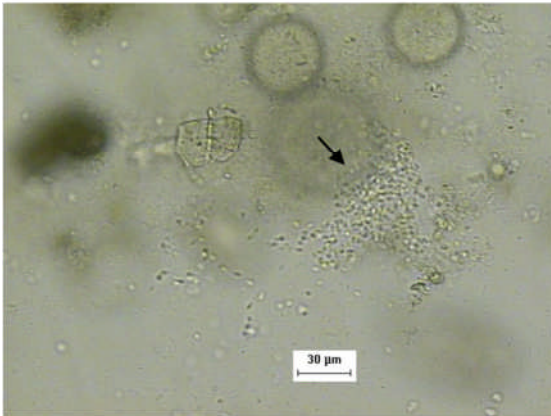
(i) Flagellates
