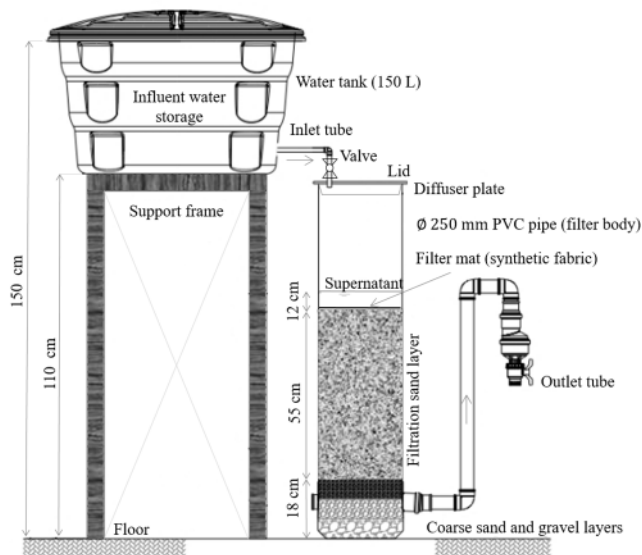
Figure 1. HSSF researched in continuous flow.
