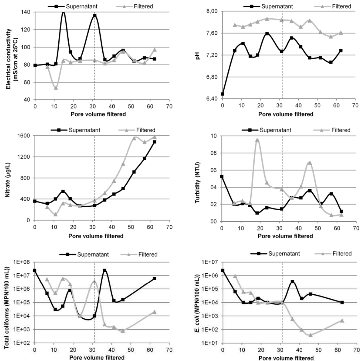
Figure 3. Filter performance adding 0.25 g/day of fish food using highly contaminated influent water during the second phase (water temperature = 24.5 \pm 0.5 °C) for twelve sequential days of operation. Vertical dashed lines indicate when the influent water was renewed.
