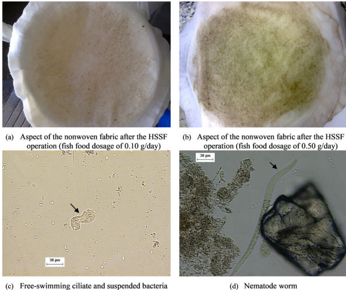
Figure 1 - Synthetic nonwoven fabrics installed on the top sand layer of the household slow sand filter (HSSF) during the first operation phase and some corresponding microscopic examinations
