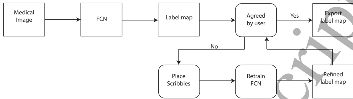
Figure 3: Framework for interactive segmentation
