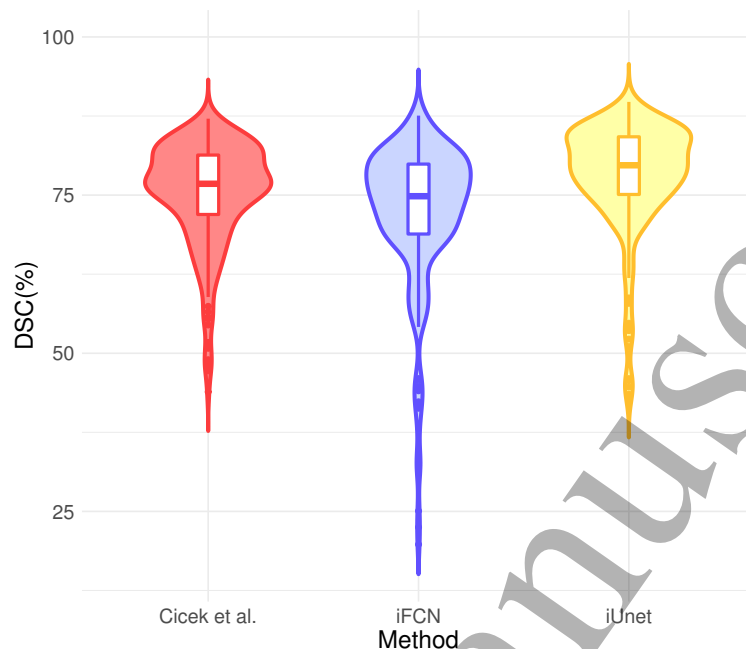
Figure 4: Performance of the Cicek et al. U-net[22], Dilated FCN network architecture and our 3D U-net in a 5-fold cross validation using dataset D1.
