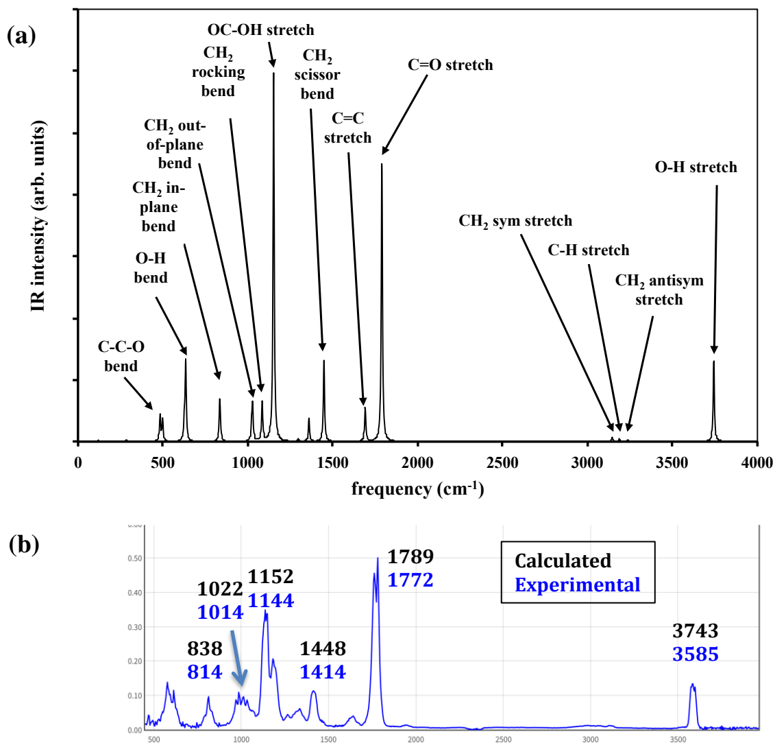
Fig. 8 (a) Calculated infrared spectrum of lowest energy conformer of acrylic acid using the B3LYP-D3/aug-cc-pVTZ method and (b) experimental IR spectrum of acrylic acid in gas phase. 33
