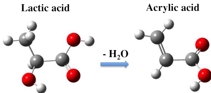
Figure 1. Figure showing the dehydration of lactic acid to acrylic acid
