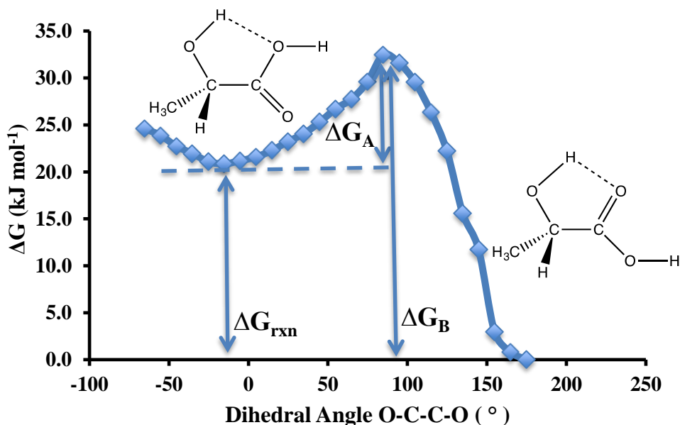
Figure 3. Relaxed dihedral scan of O-C-C-O angle of lactic acid starting with the lowest energy conformer (i.e. D) using B3LYP-D3/aug-cc-pVTZ. All coordinates were allowed to relax apart from the O-C-C-O dihedral angle.
