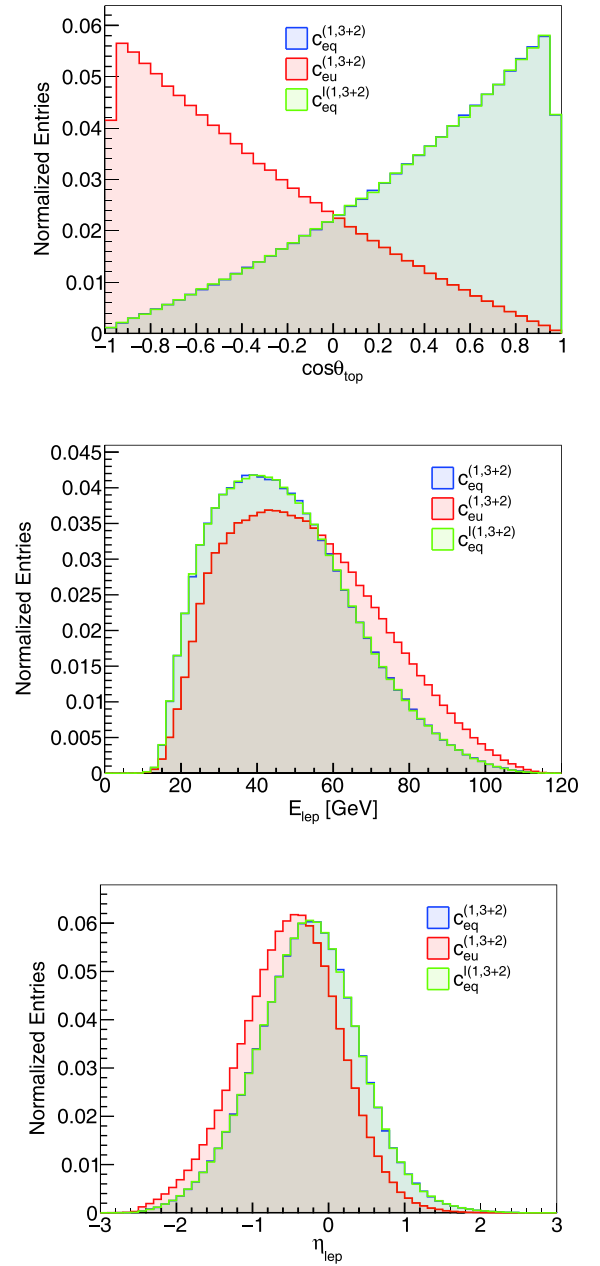
Fig. A2. (color online) Signals from c_{eq}^{(1,3+2)} , c_{eu}^{(1,3+2)} and c_{eq}^{I(1,3+2)} at the parton level. Distributions of the scattering angle, the lepton energy, and the lepton pseudorapidity are compared.
