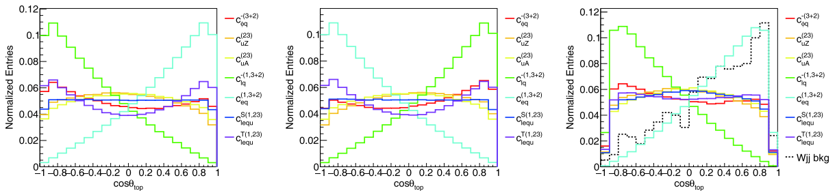
Fig. 4. (color online) Scattering angle from the signals of the seven coefficients in the first row of Eq. (27). \theta_{\text{top}} is defined as the angle between the momentum of the e^+ beam and t or \bar{t} . (left) parton level, for top production. (middle) parton level, for anti-top production. (right) reconstruction level, for top production, including the background.
