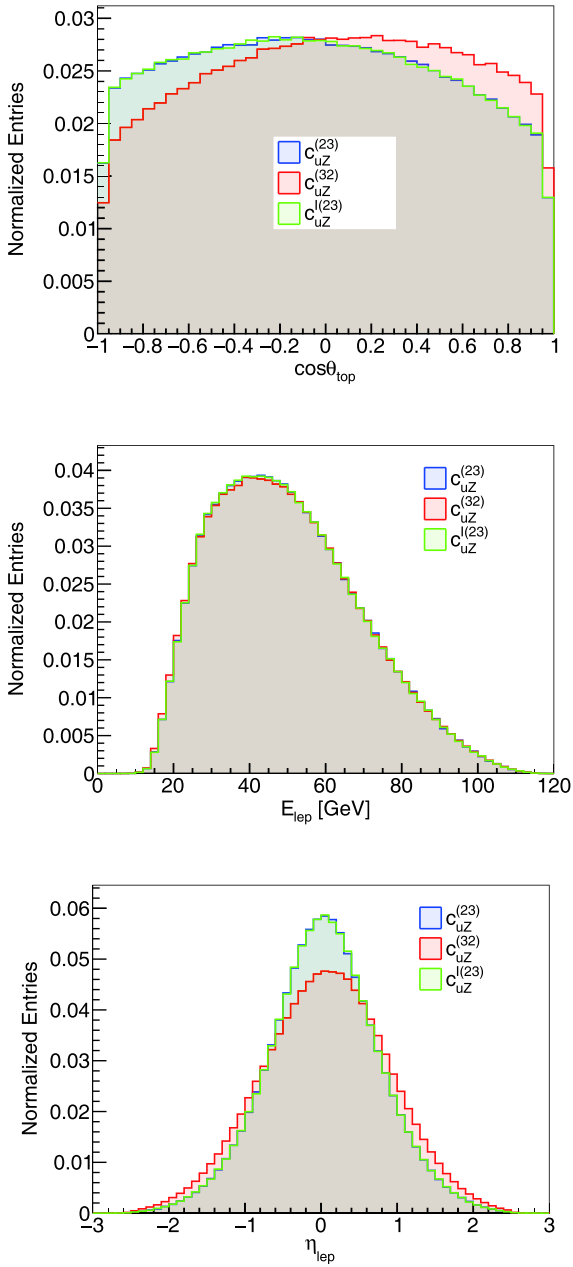
Fig. A1. (color online) Signals from c_{uZ}^{(23)} , c_{uZ}^{(32)} and c_{uZ}^{I(23)} at the parton level. Distributions of the scattering angle, the lepton energy, and the lepton pseudorapidity are compared.
