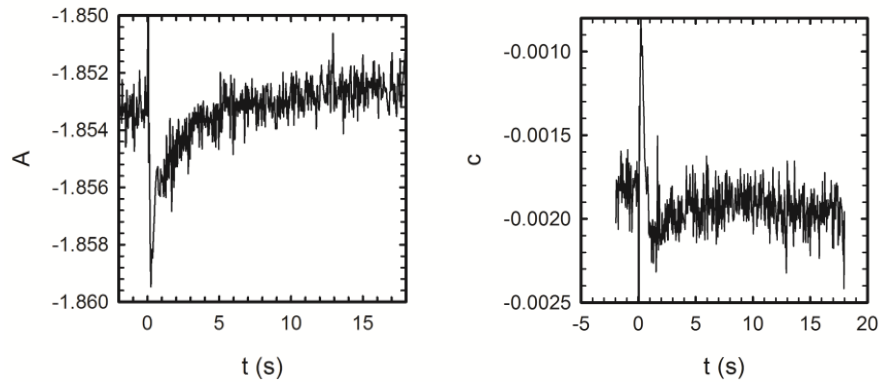
Figure 3. Modulation (left; A from Eq. 1) and residual (right, C from Eq. 1) amplitude parameters of the polarized light transmitted through the sample as a function of time for a sample of 5.0% w/w DAB in a 10.0% w/w S-811 in ZLI-1132 mixture, contained in a 10 \text{O}_m cell.
