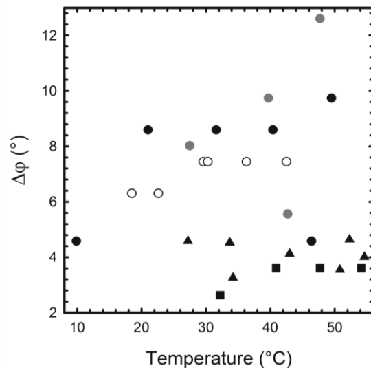
Figure 6. Phase shift amplitude for the rotation of linearly polarized light as a function of temperature for different photochromes in twisted nematic ZLI-1132 + S-811: 5.0% w/w DAB, 10.0% w/w S-811 (squares), 4.6% SO, 9.8% w/w S-811 (triangles), and for samples of 0.5% w/w N-DAB with 5.0% w/w (full circles), 11.0% w/w (empty circles) and 15.0% w/w (grey circles) S-811. The amplitude of the data for DAB (squares) was divided by 10 in order to fit in the graph scale. All samples were contained in 10 \mu m cells.
