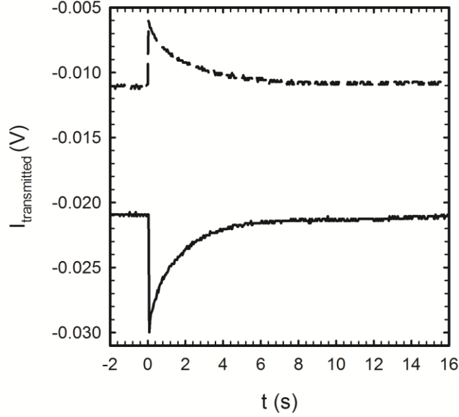
Figure 2. Typical decay curves of light transmitted through the sample, I(\theta_{an}, t) , after a flash for two different positions of the analyzer ( 90^\circ , dashed line, and 70^\circ , solid line) for a sample of 5.0% w/w DAB in a 10.0% w/w S-811 in ZLI-1132 mixture, contained in a 10 \mu\text{m} cell.
