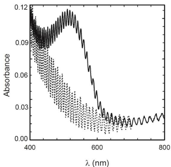
Figure 8. Absorption spectra of the open (full line) and closed (dashed line) form of AFU, for a sample of 2.1% w/w AFU in ZLI with 10.0% w/w S-811, contained in a 10 \mu m cell.
