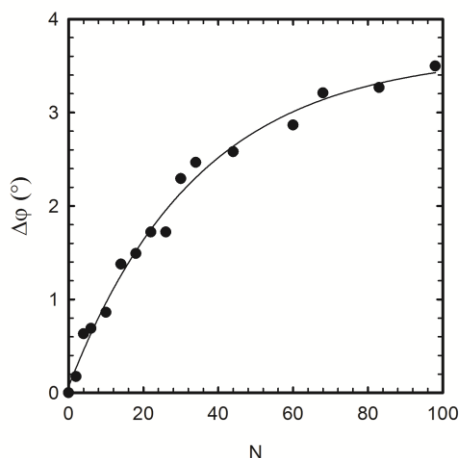
Figure 7. Phase shift amplitude, \Delta\varphi , Eq. 1., relative to the unirradiated sample, as function of the number of flashes for a sample of 8.0% w/w AB in a 9.0% w/w S-811 in ZLI-1132 mixture, contained in a 10 \text{cm} cell. The line represents the monoexponential fit to the equation in the text.
