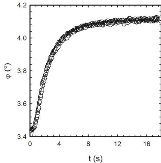
Figure 4. Phase delay decay as a function of time for a sample of 5.0% w/w DAB in a 10.0% w/w S-811 in ZLI-1132 mixture, thermostated at 57^\circ \text{C} . The line represents the
