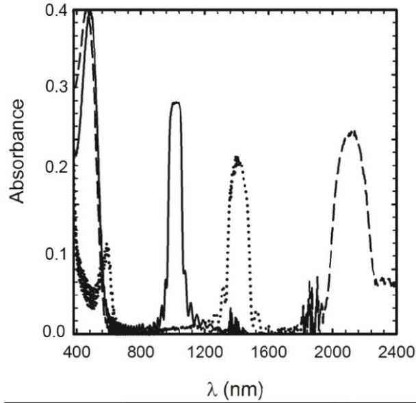
Figure 1. Absorption spectra (10 \mu m cell thickness) of samples of 0.5% w/w N-DAB in ZLI with 5.5% w/w S-811 (dashed line), 0.6% w/w N-DAB in ZLI with 11.0% w/w S-811 (full line), and 4.6% w/w SO in ZLI with 10.0% w/w S-811 (dotted line).
