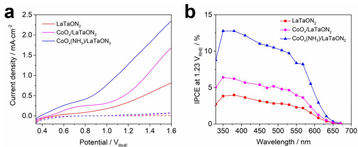
Fig. 3 Photocurrent characteristics of different CoO x -modified LaTaON 2 photoanodes (a) and comparison of IPCE for photoanodes with and without modification (b). In figure a, the J-V measurements were carried out in 1 M NaOH electrolyte (pH = 13.6) under AM 1.5 simulated sunlight (Oriol Sol3A Class AAA Solar Simulator). The dash lines show the dark-current of the corresponding LaTaON 2 photoanodes. In figure b, incident photon-to-current efficiency (IPCE) of CoO x -modified LaTaON 2 photoanodes with and without post heat treatment under NH 3 compared with the bare photoanode at 1.23 V RHE in 1 M NaOH under back-side illumination.
