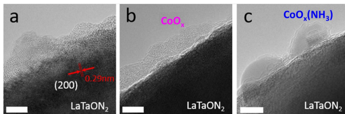
Fig. 4 HRTEM images of particles on the photoanodes. (a) A particle from an as-fabricated LaTaON 2 photoanode (PC1350). (b) A particle from CoO x /LaTaON 2 . (c) A particle from CoO x (NH 3 )/LaTaON 2 . The spacing of 0.29 nm in Figure 7a corresponding to the (2 0 0) plane of perovskite-type LaTaON 2 . The scale bars are 5 nm.
