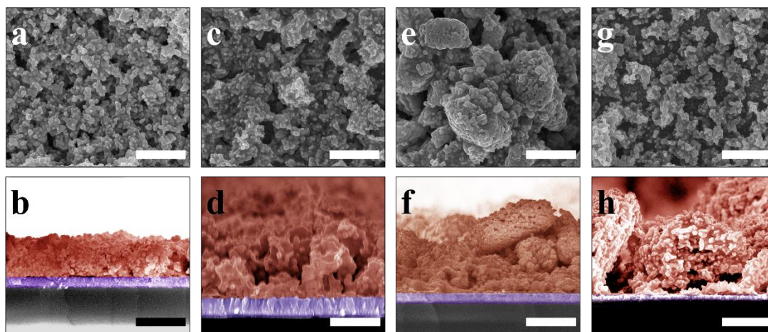
Fig. 1 SEM images of the particle-assembled photoanode films. The top row shows the surface of the photoanodes, while the bottom shows the corresponding cross sections. The scale bars are 2 \mu\text{m} . (a) and (b): PC1150; (c) and (d): PC1250; (e) and (f): PC1350; (g) and (h): PC1450.
