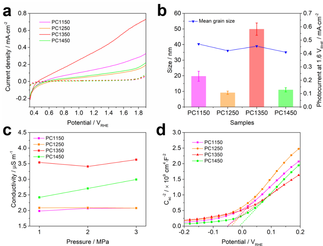
Fig. 2 Photocurrent characteristics of LaTaON 2 photoanodes (a). The J-V measurements were carried out in 1 M NaOH electrolyte (pH = 13.6) under visible-light irradiation (a 500 W xenon lamp with a Hoya L-42 cut-off filter, \lambda \geq 420 nm). The scan rate was 30 mV/s. The dash lines show the dark-current of the corresponding LaTaON 2 photoanodes. Comparison of various samples and their corresponding photocurrents at 1.6V RHE (b). The average (filled bars) photocurrents at 1.6 V RHE were extracted from the J-V measurements. The curve with blue inverted triangles stands for the mean grain sizes. Bulk electrical conductivity of LaTaON 2 powders under given pressures (c). Comparison of various LaTaON 2 samples with their corresponding flat band potentials and carrier densities (d). The Mott-Schottky tests were conducted in the dark with 1 M NaOH served as electrolyte. The frequencies were 1000 Hz, and the penetration amplitudes were 5 mV.
