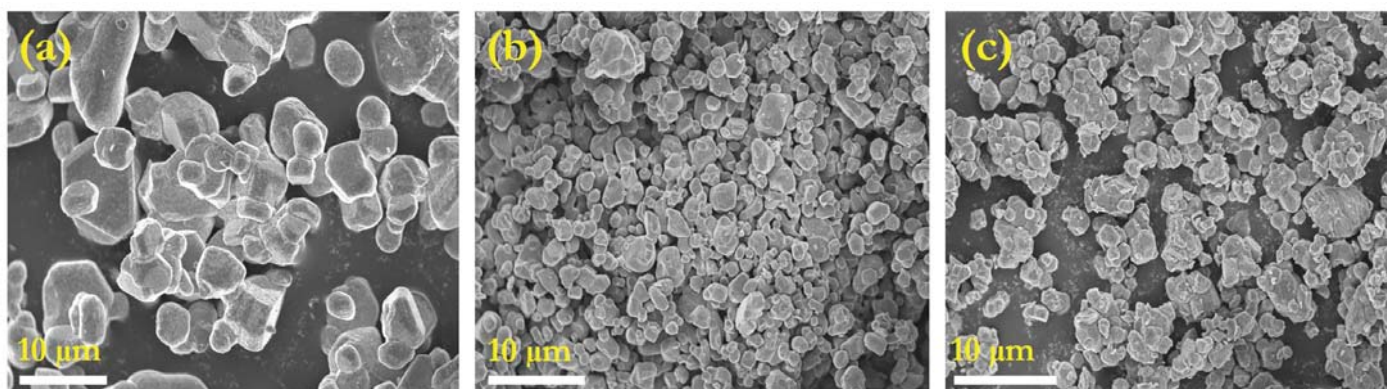
Fig. 3 (a) SEM micrograph of (a) LRO (b) LRTO (c) LRFO
