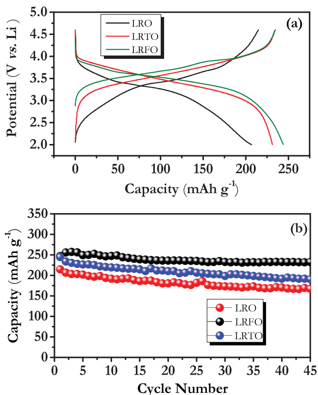
Fig. 5 Galvanostatic charge discharge profile of LRO,LRTO and LRFO; (b) Cycle Number vs. Capacity for LRO, LRFO and LRTO for the first 45 cycles
