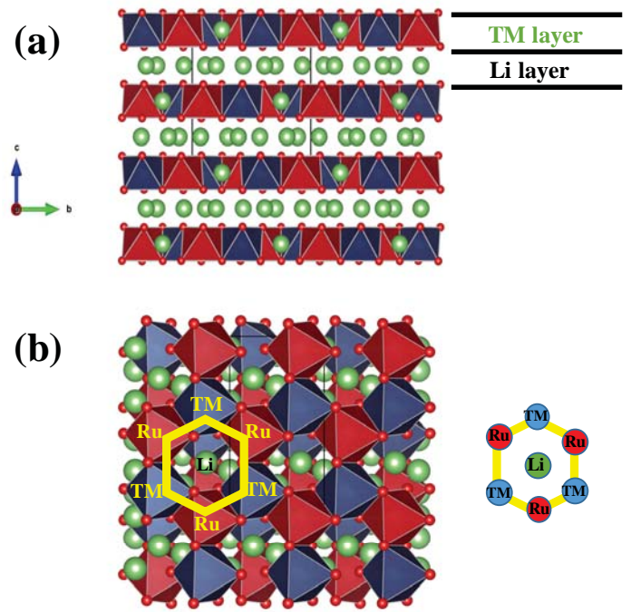
Fig. 1 Crystal structure of LLCs as viewed from the; (a) a axis indicating alternate layers of TM and Li layers; (b) c axis indicating the arrangement of Ru and substituted TM metals in a hexagonal network (yellow) around Li (TM can be Ti, Sn and Fe). The 3d TM and Ru atoms are distributed in a 1:1 ratio to clearly indicate the hexagonal network around Li. A more realistic visualisation would be to have 3d TM randomly occupy a quarter of the original Ru sites.
