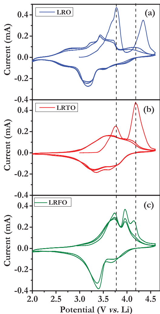
Fig. 4 CV trace recorded for the first two cycles at 0.1 \text{ mV s}^{-1} between 2- 4.6 V vs. Li (a) LRO, (b) LRTO and (c) LRFO
