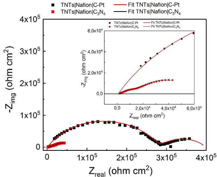
Figure 3: Nyquist plot of the two SSPEC cell configurations at 0.5 V vs. cathode and photocathode respectively, under 1 Sun illumination. Anode was provided with wet air (80% RH) and the (photo)cathode with dry Ar. Inset: Fitted data in the high frequency domain.
