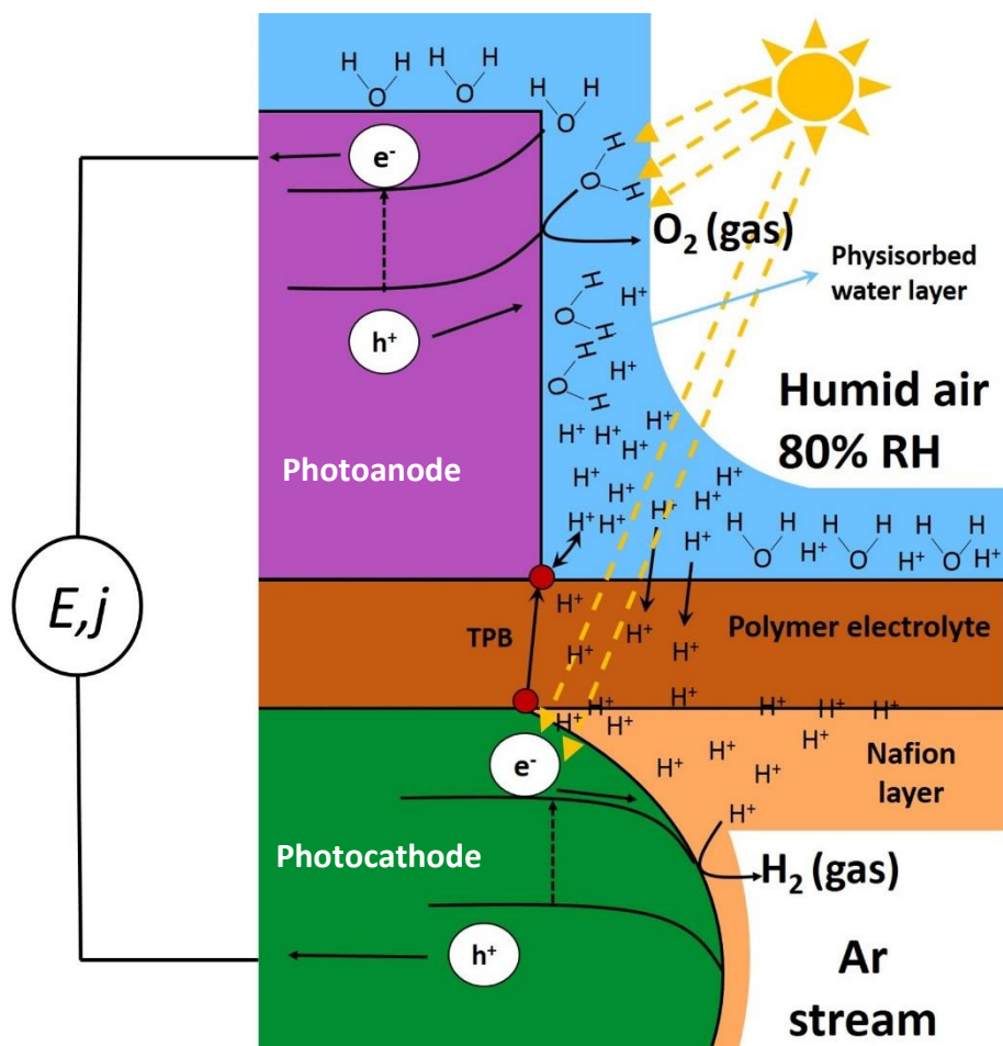
Figure 4: The concept of water vapor splitting and hydrogen production in a tandem-SSPEC cell. The surface water layer on the photoanode contributes to the proton transport towards the Nafion® membrane, while the lighter brown area in the photocathode represents the Nafion® layer, which apart from proton conduction, acts a binding agent. The photogenerated electrons in the photoanode are recombined in the external circuit with the photogenerated holes in the photocathode. In the case of the SSPEC cell, the photocathode is replaced by Pt nanoparticles, which are the catalysts for proton reduction and hydrogen evolution under the same conditions. The separating Nafion® membrane and the Nafion® layer are transparent.
