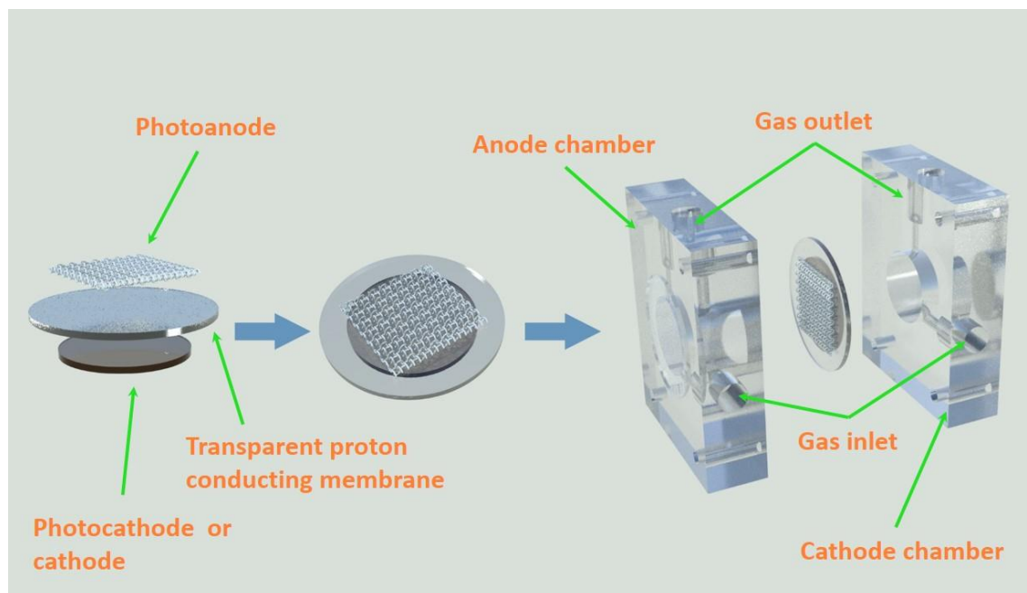
Figure 1: Schematic representation of the construction of the button-like PEC membrane, as well as its mounting on the custom-made solid-state PEC device. The PEC membrane is sandwiched between two silicone O-rings, which have appropriate copper wiring for connection to the potentiostat. The PEC device is of continuous flow type.
