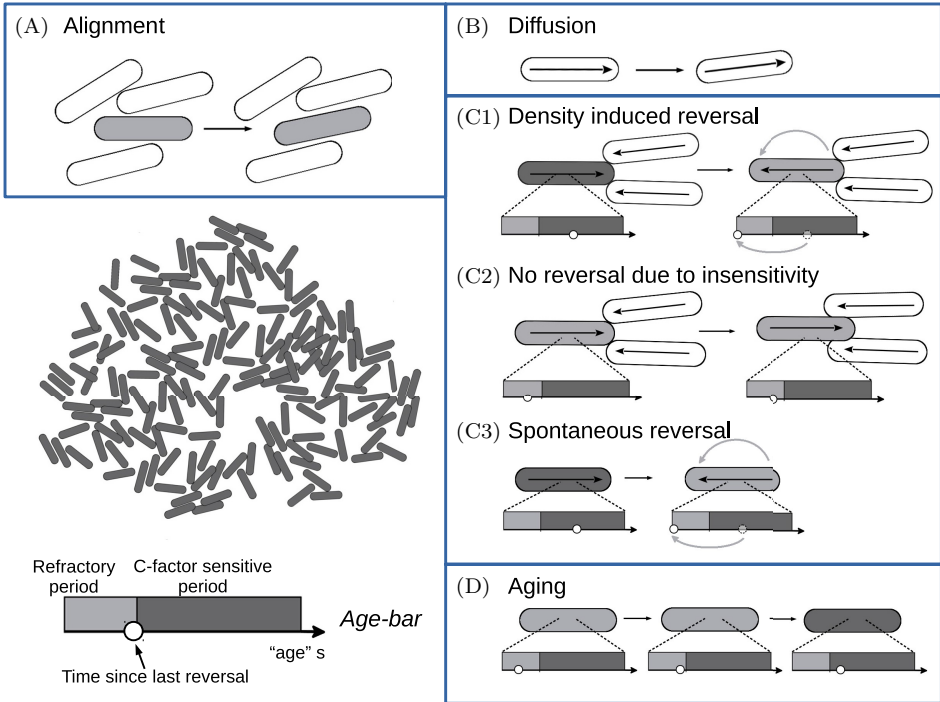
Fig. 1. Ingredients of the memory-dependent myxobacteria model. (A): Nematic Alignment. The bacterium depicted in gray aligns nematicly with its neighbors due to steric interactions and size exclusion effects. (B): Angular Noise. The bacterium's orientation is subject to random fluctuation. (C/D): Reversals and Aging. Bacteria can either be insensitive to C-signaling (light gray) or sensitive (dark grey). The age bar (explained in the lower, left corner) depicts the two periods and the bacterium's current state (white dot). Upon meeting oppositely moving bacteria, a bacterium can reverse, if sensitive to C-signaling (C1) or not, if in the refractory period (C2). They can also reverse spontaneously (C3). Insensitive bacteria age into a sensitive state (D) and reversals reset their age variable to zero (C1 and C3).
