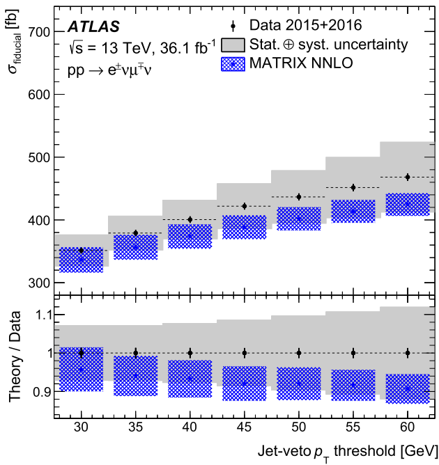
Fig. 6 Comparison of the measured fiducial cross-section as a function of the jet-veto p_T threshold with various theoretical predictions. The measurement is compared with NNLO predictions from MATRIX on the left. This calculation does not include the NLO EW correction and is Born-level, whilst the measurement is conducted using dressed leptons, which might account for some of the differences seen. On the right a comparison with NLO+PS predictions from POWHEG-BOX+PYTHIA 8, POWHEG-BOX+HERWIG++ and SHERPA 2.2.2 for q\bar{q} initial states, com-
