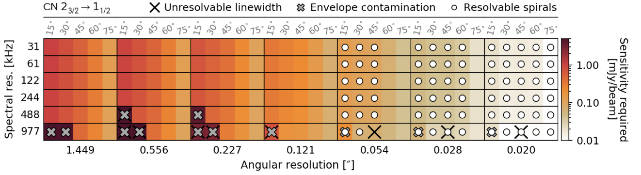
Figure 15. Same as Fig. 10 but for \text{CN } 2_{3/2} \rightarrow 1_{1/2} .
