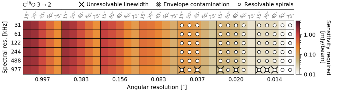
Figure 12. Same as Fig. 10 but for \text{C}^{18}\text{O } 3 \rightarrow 2 .
