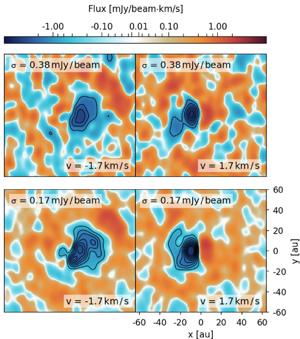
Figure 18. Channel maps for \text{SO } 6_7 \rightarrow 5_6 indicating whether spiral structure can be visually distinguished for two different sensitivities; the lower sensitivity is the noise we determined is necessary to detect the spirals, whereas the higher sensitivity is the noise required to detect the contrast between and arm and inter-arm regions. The contours indicate levels of 4\sigma and the bottom-right panel indicates the physical scale of the observed disc model, which is constant across all transitions shown.
