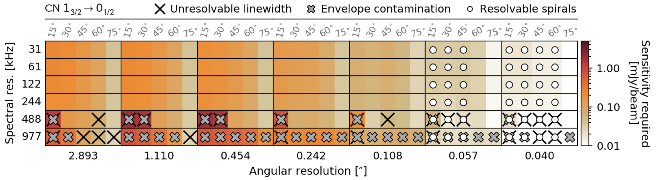
Figure 16. Same as Fig. 10 but for \text{CN } 1_{3/2} \rightarrow 0_{1/2} .
