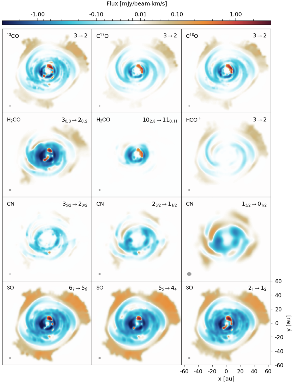
Figure 8. Noise-free integrated intensity maps (integrated from -5.0 to -0.8 \text{ km s}^{-1} and from 0.8 to 5.0 \text{ km s}^{-1} ) for each molecular transition, for an inclination of 15^\circ , a channel spacing of 31 \text{ kHz} and the ‘out28’ antenna configuration. The bottom-right panel indicates the physical scale of the observed disc model, which is constant across all transitions shown. The grey circle in each panel shows the beam size for the corresponding observation, but note that the level of detail shown here is not currently attainable with ALMA. For comparison purposes, the corresponding column density maps can be found in Paper I .
