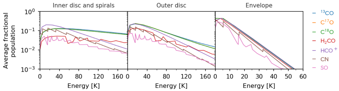
Figure 7. Fractional energy-level populations averaged over grid points within the inner disc and spirals (left-hand panel), the outer disc (middle panel), and the envelope (right-hand panel). The disc regions are determined by density ranges.
