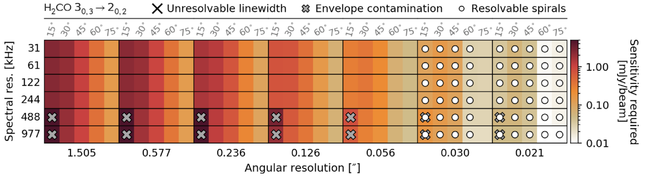
Figure 13. Same as Fig. 10 but for \text{H}_2\text{CO } 3_{0,3} \rightarrow 2_{0,2} .
