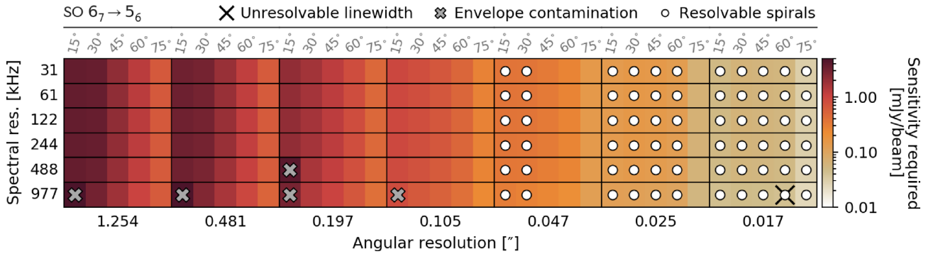
Figure 17. Same as Fig. 10 but for \text{SO } 6_7 \rightarrow 5_6 .
