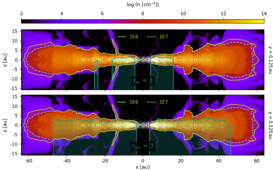
Figure 2. Nuclei number densities of the disc model along the y = 0.125 au plane with solid and dashed green lines overplotted at number densities that approximately demarcate the boundaries of LTE validity. The teal lines show the boundary where \tau = 3 at a frequency of 90 GHz (top) and 850 GHz (bottom); hence, the shaded regions indicate the optically thick regions of the disc when viewed from above. The white dots indicate the x and z positions of all of the fluid elements (i.e. not only those constrained to y = 0.125 au) that are chemically processed (see Paper I).
