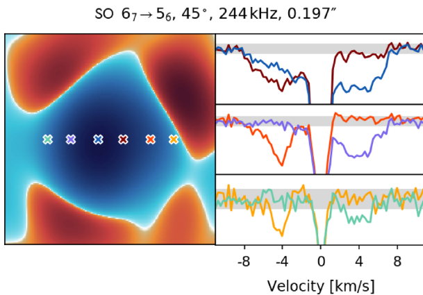
Figure 20. Integrated intensity map of \text{SO } 67 \rightarrow 56 with an on-source observation time of 2.5 h. Overlaid are crosses denoting the positions of molecular spectra extraction, and these extracted molecular spectra are displayed below the intensity map for a spectral resolution of 244 kHz, normalized against the non-envelope flux minima and maxima. The grey regions in the spectra plots denote the noise level, which is 1.24 \text{ mJy beam}^{-1} .
