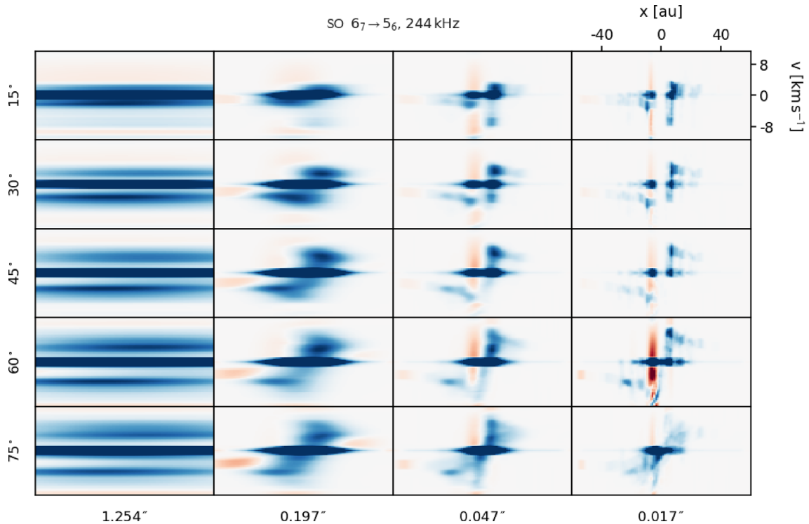
Figure 21. Position-velocity diagram for SO 6_7 \rightarrow 5_6 across different disc inclinations and beam sizes, for a spectral resolution of 244 kHz. The top-right panel indicates the position and velocity ranges of the observed disc model, which are constant across all panels.
