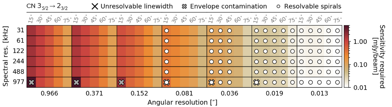
Figure 14. Same as Fig. 10 but for \text{CN } 3_{5/2} \rightarrow 2_{3/2} .
