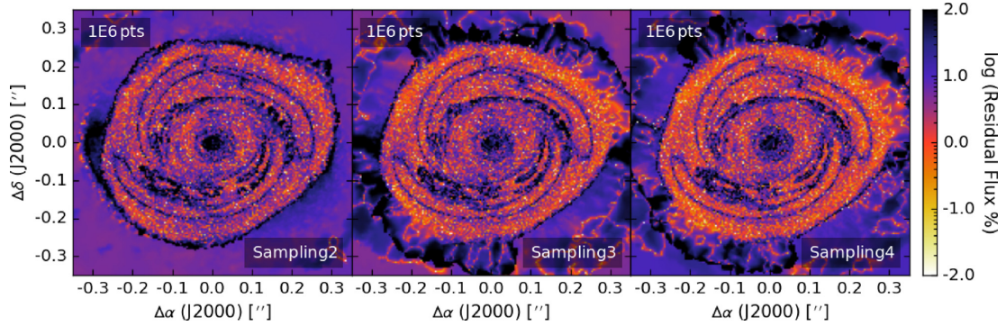
Figure 4. Residual integrated line flux for \text{C}^{17}\text{O } 1 \rightarrow 0 calculated under the assumption of LTE, between two LIME runs using the indicated number of grid points, with standard sampling (left), a model-specific sampling routine (middle), and a model-specific sampling routine with an optical depth surface to constrain the positioning of grid points (right). We define this residual as |(f_1 - f_2)/(f_1 + f_2)| , where f denotes integrated flux per pixel.
