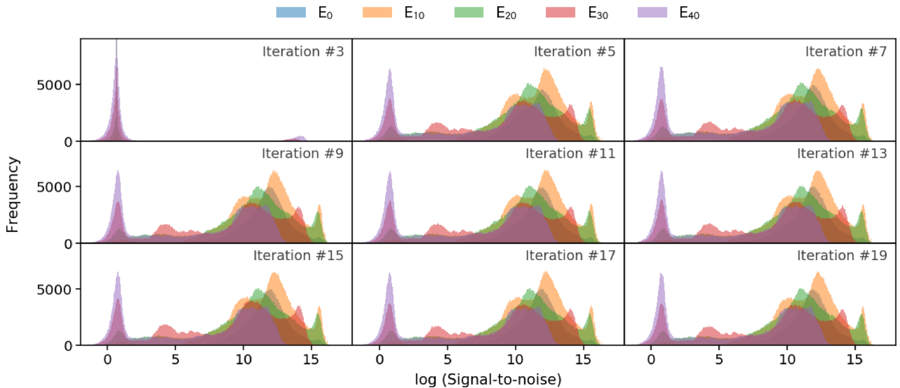
Figure A1. Histograms of the signal-to-noise ratios of different energy levels (i.e. J number) for C^{17}O\ 1 \rightarrow 0 as the amount of iterations of level population calculations increases. A converged distribution is reached by five iterations. The non-LTE LIME run shown here uses 1 \times 10^6 grid points and Sampling2.
