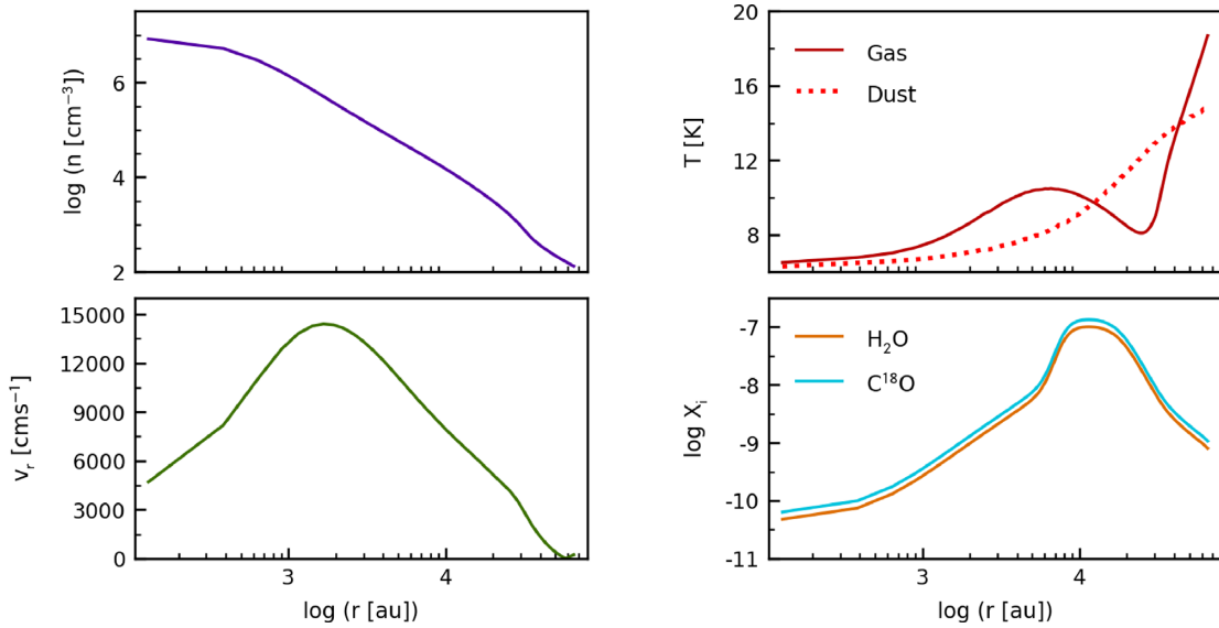
Figure 1. Spherically symmetrical envelope model used in the radiative transfer calculations (Keto, Caselli & Rawlings 2015).
