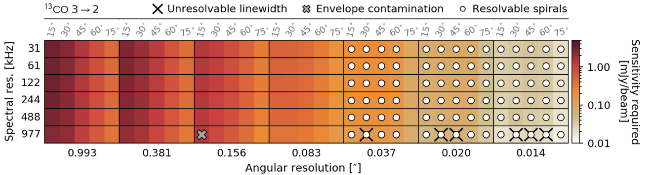
Figure 10. Sensitivity needed to detect ^{13}\text{CO } 3 \rightarrow 2 line flux across different combinations of angular resolution (i.e. antenna configuration), spectral resolution, and disc inclination (grey labels). The white circles indicate whether the spirals can be, in theory, spatially resolved, which is determined by eye from noise-free flux maps. The thick grey crosses indicate combinations that result in line spectra that are indistinguishable from the envelope. The thin black crosses indicate combinations where the Gaussian fitted to the line spectra (see Fig. 9) is not spectrally resolvable.
