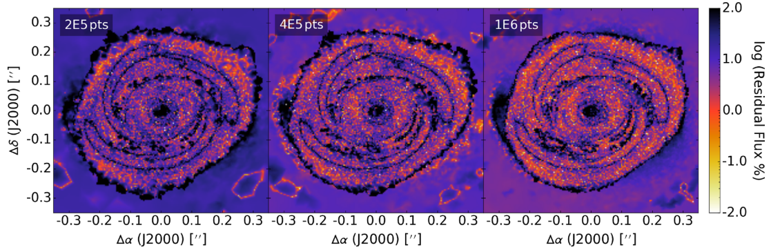
Figure 3. Residual integrated line flux for \text{C}^{17}\text{O } 1 \rightarrow 0 calculated under the assumption of LTE, between two LIME runs using the indicated number of grid points, with standard sampling. We define this residual as |(f_1 - f_2)/(f_1 + f_2)| , where f denotes integrated flux per pixel.
