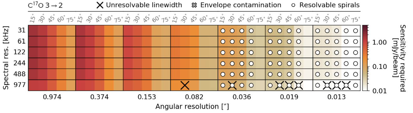
Figure 11. Same as Fig. 10 but for \text{C}^{17}\text{O } 3 \rightarrow 2 .
