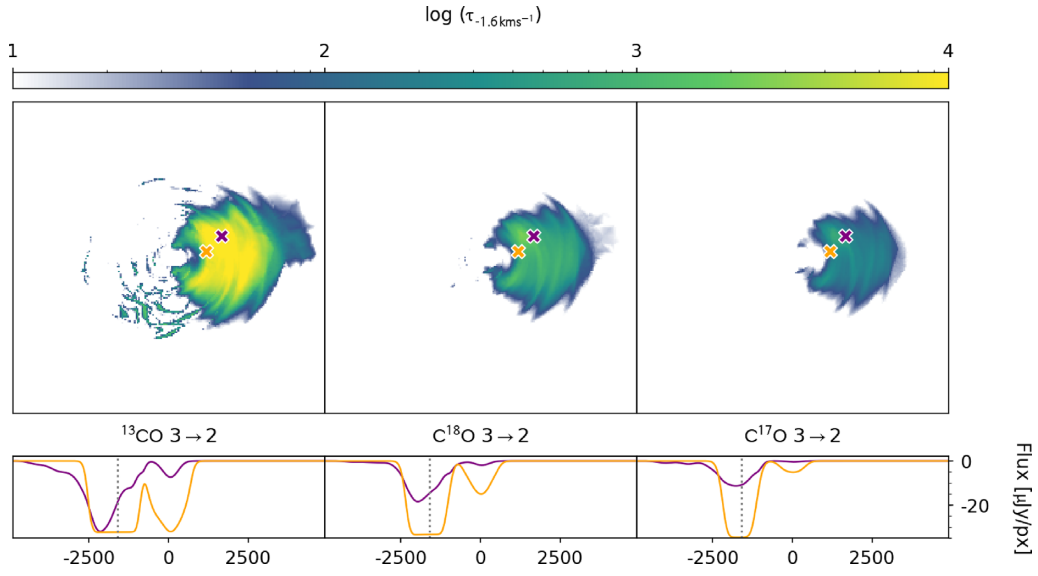
Figure C2. Same as Fig. C1 but for different CO isotopologues absorption.
