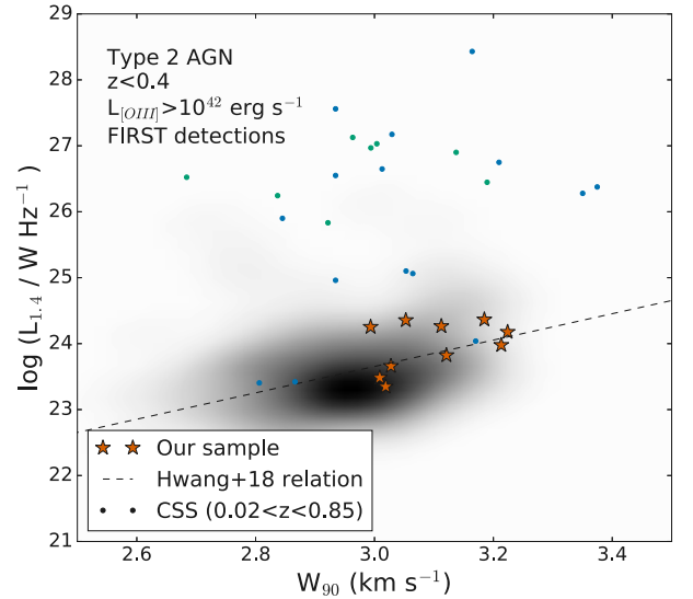
Figure 12. The width of the [O III] line ( W_{90} ) as a function of radio luminosity. The grey scale shows the underlying distribution of type 2 AGN (Mullaney et al. 2013) with z < 0.4 and a luminosity cut of L_{[\text{O III}]} > 10^{42} erg s ^{-1} (i.e. the selection criterion of our sample; Fig. 1) that are detected in FIRST. A similar selection criterion was used by Hwang et al. (2018), using the z < 0.8 quasars from Zakamska & Greene (2014), to produce the relationship shown by the dashed line. Our sample is shown as the red stars, where W_{90} is measured from our GMOS data in a 3 arcsec aperture (approximating the SDSS fibre). The circles mark the CSS radio AGN from Holt et al. (2008; green; using the FWHM of their single Gaussian component fits), and Gelderman & Whittle (1994; blue). Our sources have more representative radio luminosities compared to CSS radio galaxies; however, we have shown that they also contain compact radio jets. Consequently, radio jets should be explored as a crucial feedback mechanism for all quasars.
