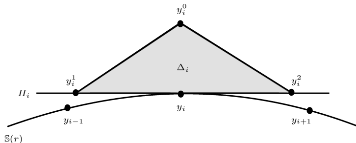
Figure 1: Construction of the simplices \Delta_i .
