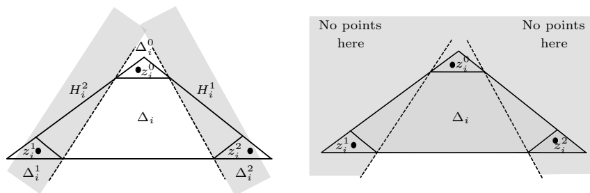
Figure 2: The simplices \Delta_i^j , the points z_i^j and the half-spaces H_i^j (left). Illustration of the events A_i (right).
