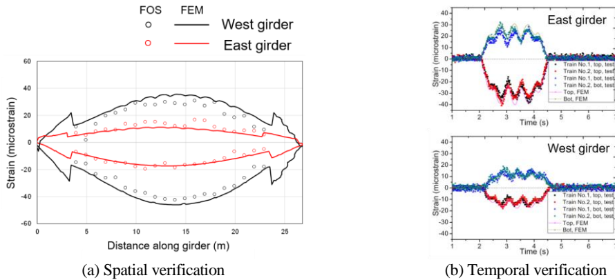
Figure 3. Physics-based approach (adapted from [6])
