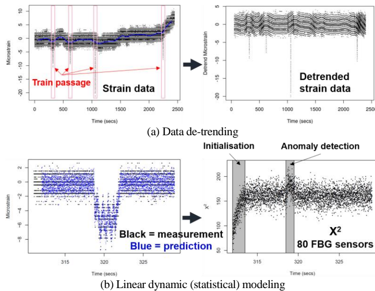
Figure 4. Data-driven approach (adapted from [9])
