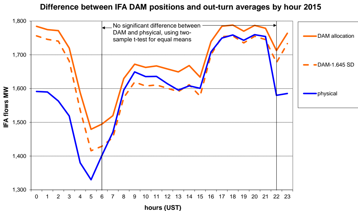
Figure 7. Difference between DAM positions and out-turn averages by hour (UST) for 2015.
