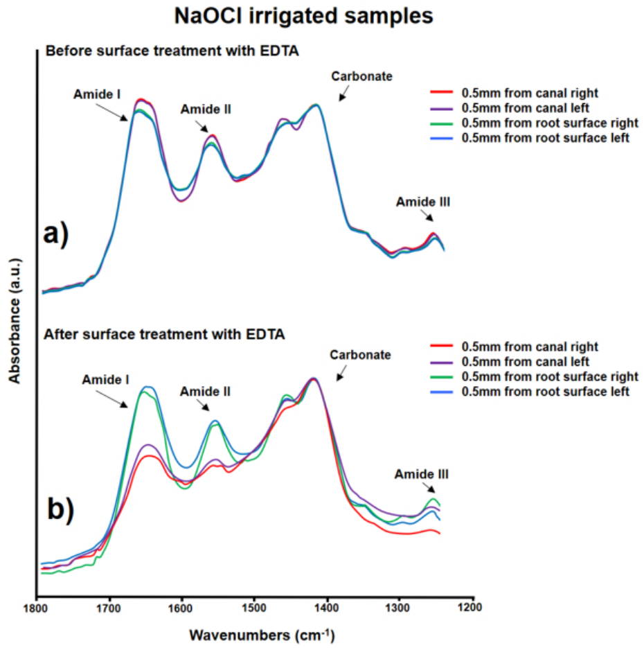
Figure 2. Overlaid spectra for a NaOCl irrigated sample (a) before and (b) after surface treatment with EDTA.
