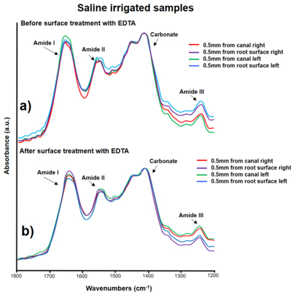
Figure 1. Overlaid spectra for a saline irrigated sample (a) before and (b) after surface treatment with EDTA.
