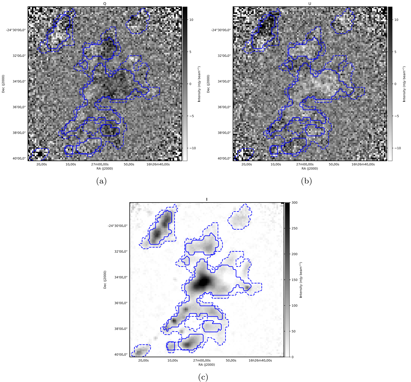
Figure 1. (a–c) POL-2 Stokes Q , U , and I maps of the Oph-C region, respectively. The intensity is shown in gray scale. The ASTMASK and the PCAMASK used in the data reduction process are shown with dashed and solid lines, respectively.
