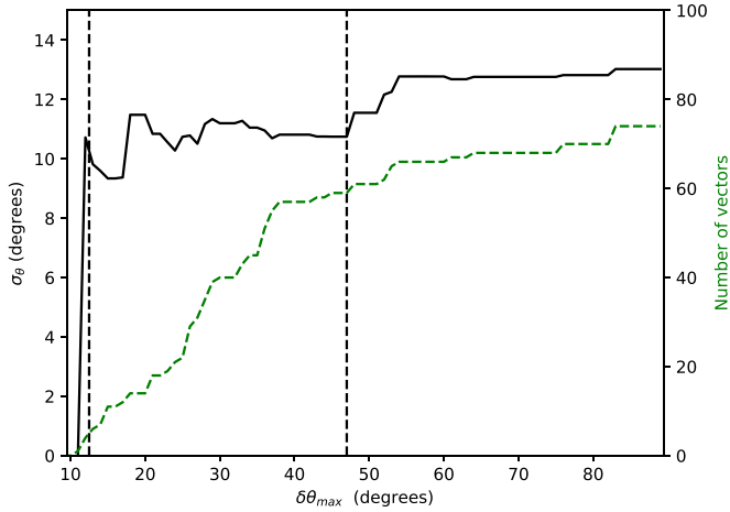
Figure 10. Left-hand axis: \sigma_{\theta} as a cumulative function of \delta\theta_{\text{max}} , shown by the black solid line. Right-hand axis: number of vectors (green dashed line) included in the cumulative function. The average standard deviation is measured over the region between two black dashed lines.
