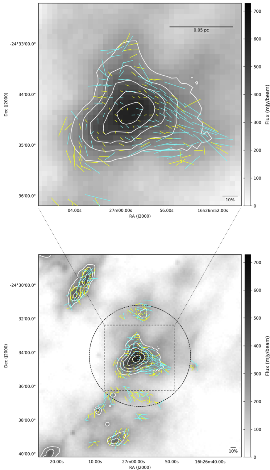
Figure 3. Magnetic field orientation maps. The total intensity of the 850 \mu\text{m} continuum from the GBS project is shown in gray scale. The total intensity is also shown in contour levels, starting from 250 \text{ mJy beam}^{-1} and continuing at steps of 80 \text{ mJy beam}^{-1} . Vectors are from the POL-2 data with \delta P < 5\% . The yellow and cyan vectors correspond to data with P/\delta P > 2 and P/\delta P > 3 , respectively. A reference 10% vector is shown in the lower right corner. A black dashed circle shows the central region of 3' radius.
