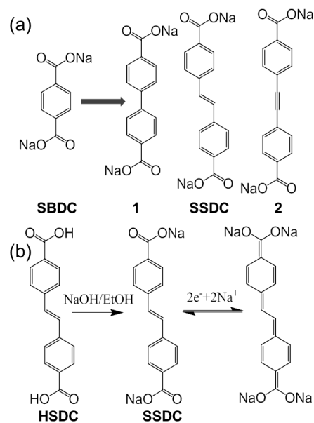
Figure 1. (a) Schematic chemical structure of starting molecule SBDC and three possible linkages to extend its \pi -conjugation, forming 1, SSDC and 2 respectively; (b) schematic diagram for the synthesis and reversible Na-ion insertion/extraction mechanism of SSDC.
