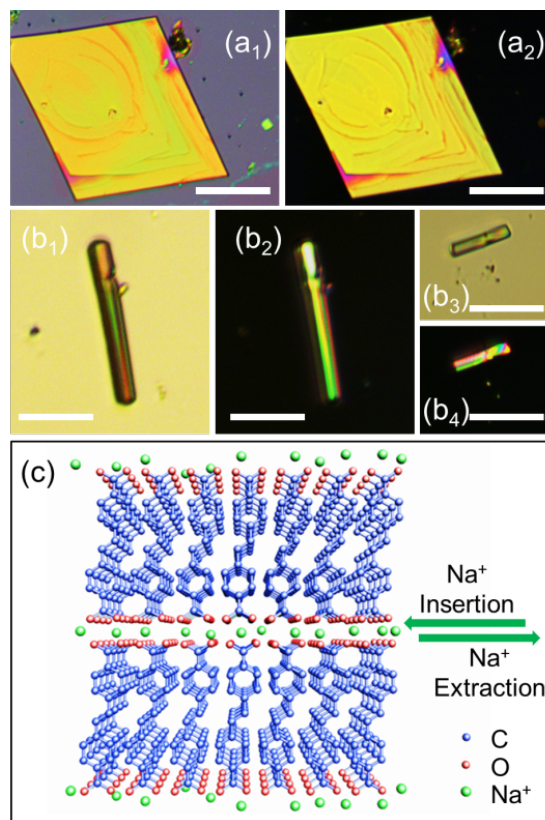
Figure 3. (a 1 ) photo image and (a 2 ) corresponding cross-polarized light microscopy (PLM) image of a typical SSDC crystal; (b 1 , b 3 ) photo images and (b 2 , b 4 ) their corresponding cross-polarized light microscopy images of typical SBDC crystals. The uniform brightness of PLM images of SSDC and SBDC suggest that the self-assembly crystals are single crystalline. Scale bar: 30 \mu\text{m} . (c) schematic molecular packing of SSDC: the molecules are stacking layer-by-layer with strong \pi - \pi intermolecular interaction in plane and carboxylate group situated on the surface of the layers, forming a channel exactly at the active center for insertion/extraction of Na ions between layers.
