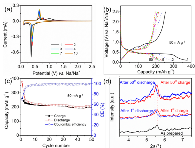
Figure 4. (a) typical CV curves of SSDC films in the first 10 cycles; (b-c) Electrochemical performances of SSDC: (b) voltage profiles (1 st , 2 nd , 5 th , 10 th , 20 th and 50 th cycles are selected as representatives), (c) cycleability; (d) XRD patterns of as-prepared SSDC films and XRD patterns of SSDC films after discharging to 0.1 V (vs. Na/Na + ) and after charging to 2.5 V (vs. Na/Na + ).
