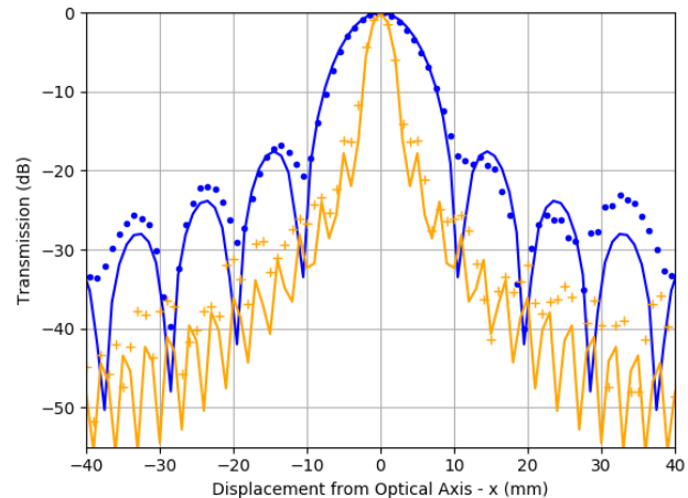
Fig. 9. x-axis beam cuts, at the nominal focus position of 230mm, for 116 GHz blue dots and 290GHz orange cross. The expected Airy profiles for each are shown as continuous lines.
