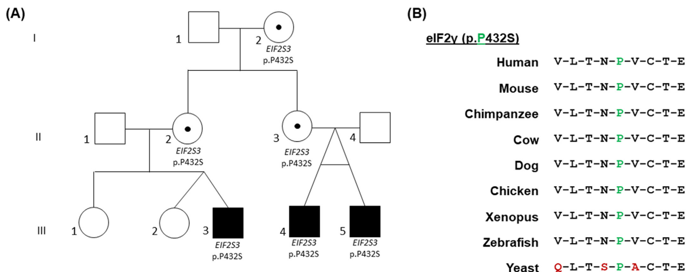
Fig. 2. (A) Pedigree 1 harbouring the EIF2S3 (p.Pro432Ser) variant. This pedigree consists of three affected individuals that are hemizygous for the EIF2S3 (p.Pro432Ser) variant, represented by the black shaded squares labelled with ' EIF2S3 p.Pro432Ser'. Patients III 4 and III 5 are monozygotic twins. The circles containing a dot highlight the females that carry the variant in heterozygous form. Unshaded squares/circles represent males and females that were negative for the variant respectively. The roman numerals on the left of the image depict the generation within the pedigree. The numbers '1' – '5' distinguish between each individual within that generation, which are referred to in the text. (B) Conservation of the substituted eIF2 \gamma residue. Conservation of the P432 amino acid (highlighted in green) that is substituted in Pedigree 1. Amino acids that differ from the human WT protein sequence are highlighted in red (only in the yeast sequence). The surrounding protein sequence in eIF2 \gamma is very highly conserved across multiple species.
