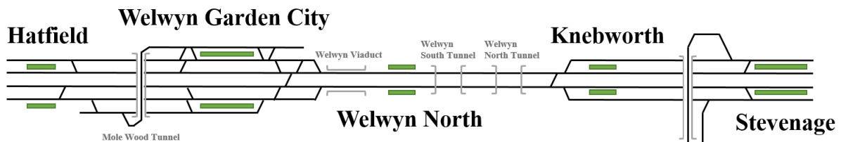
Fig. 2 – Infrastructure layout of the considered network
