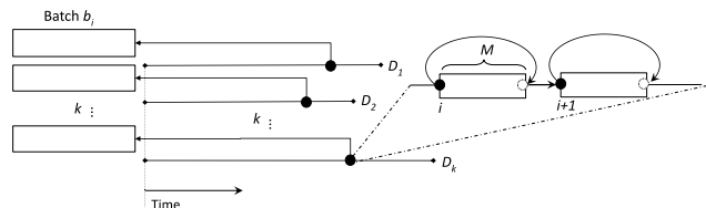
FIGURE 3. Batch formation for LSTM-RNN training from multiple videos. Feature vectors are extracted from temporal windows of length M . The windows move by M frames at each new batch to form b_j . D_k denotes the k^{th} training video.
