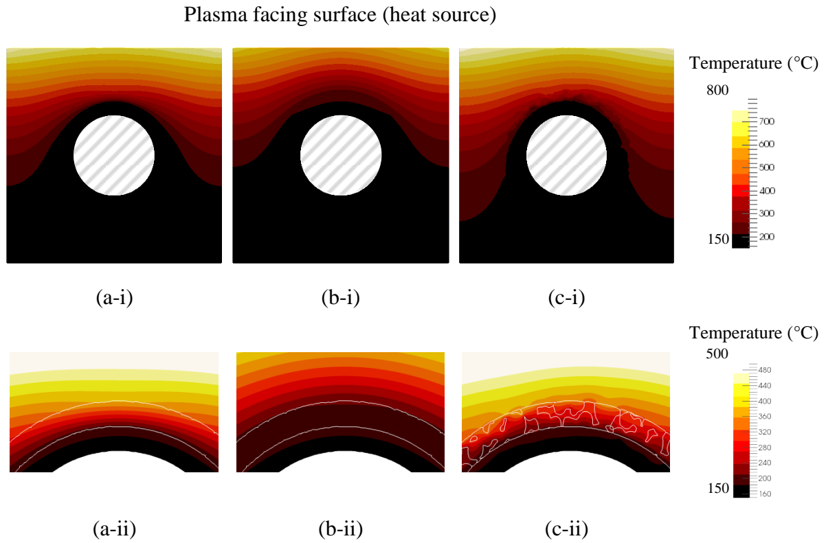
Figure 19. Temperature contour map on front view of monoblock once steady state had been reached for (a) CAD_{anisotropic} , (b) CAD_{isotropic} and (c) IBFEM simulations.
