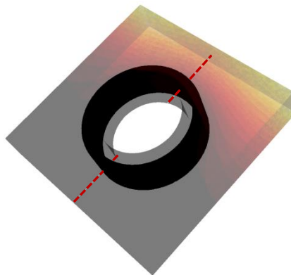
Figure 20. Visualisation of monoblock (armour and pipe sections semi-transparent) to show temperature profile path.
