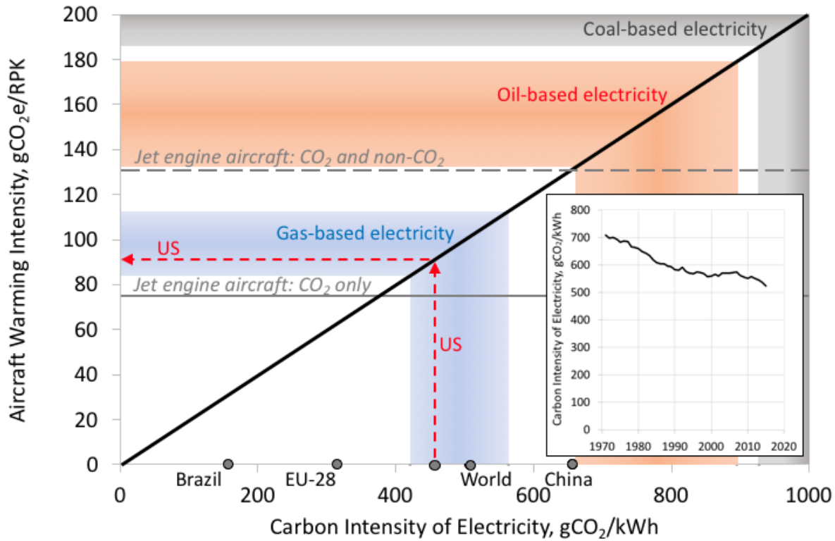
Fig. 1. Warming intensity of a projected first-generation all-electric aircraft and of a current-generation jet engine aircraft versus carbon intensity of electricity. The mission length is 400 nmi (741 km). The lifecycle CO 2 intensity of the all-electric aircraft with an electricity intensity of 180 Wh/RPK is based on a design in [18] and takes into account efficiencies of 95% for battery charging and 95% for electricity transmission/distribution. In contrast, the lifecycle CO 2 intensity of the A320neo of 75 gCO 2 /RPK is based on an energy intensity of 0.9 MJ/RPK, calculated with the aircraft performance model Piano-X [40], and a well-to-tank efficiency of 88% [41]; its warming intensity corresponds to two times its direct CO 2 emissions. The shaded areas represent the interquartile range of the CO 2 intensity of coal (limited to 1,000 gCO 2 /kWh), oil, and natural gas-based electricity on a country basis in 2015 [2]. The 2015 electricity fuel mix in Brazil, the EU-28, the US, and the world average would lead to a lower warming intensity of all-electric aircraft compared to jet engine aircraft (two times the CO 2 intensity), as exemplified by the
