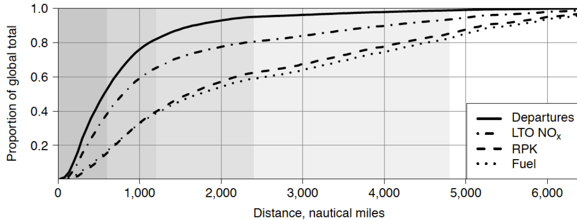
Fig. 4. Cumulative distributions of key operational variables by the global commercial aircraft fleet in 2015. The variables consist of departures, NO x emissions at landing and takeoff (LTO), revenue passenger-km (RPK), and fuel consumed. The flight distances of multiples of 600 nmi (1,111 km) are shown in terms of shaded areas. Full adoption of an all-electric aircraft with a range of 600 nmi would account for half of all aircraft departures and for 15% of all RPK. It would reduce one-third of all narrow-body related LTO NO x emissions and 15% of global narrow-body jet fuel use. Extending the range to 1,200 nmi (2,222 km) would significantly increase the impact. All numbers were derived with the Aviation Integrated Model AIM2015 [39].
