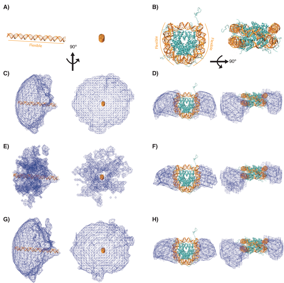
Figure 10: Cartoon representation of A) 60 bp B-DNA, and B) NCP molecule. Protein molecules are colored in cyan and DNA molecules are colored in orange. The flexible regions sampled in MC simulations are highlighted by lines. C) and D) density plot of spatial coverage of MC ensemble. E and F) density plot of the spatial coverage of subsampled ensemble. G) and H) density plot of the spatial coverage of TAMD ensemble. 90 degree rotation about the z-axis is shown for each case.
