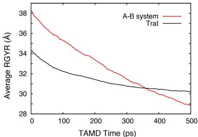
Figure 5: Averaged RGYR calculated from TAMD simulations of A-B system (red) and TraI protein (black).
