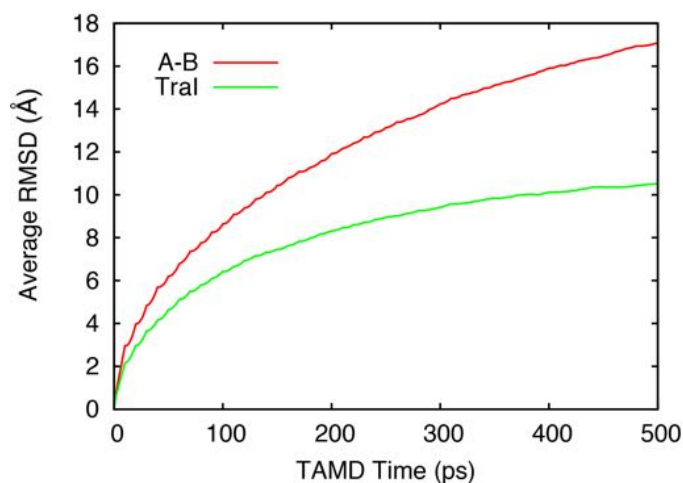
Figure 4: Red: Averaged backbone RMSD calculated from 175 independent TAMD simulations of A-B system. RMSD are calculated by aligning domain A. Green: Averaged backbone RMSD calculated from 155 independent TAMD simulations of TraI protein. RMSD are calculated by aligning the first domain (residue 1-192).
