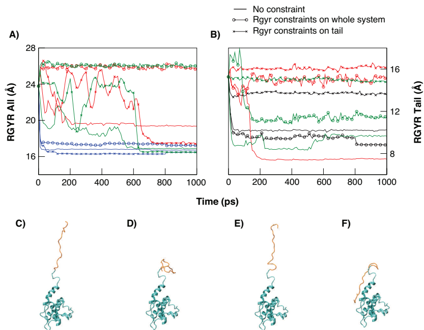
Figure 8: Affect of RGYR constraints on A-tail TAMD simulations. A). RGYR plot of the entire A-tail system (residues 1-143) from three representative TAMD simulations. B). RGYR plot of tail region (residues 123-143) from three representative TAMD simulations. For both panels A and B straight lines without symbols indicate the TAMD simulations without constraints; lines with circles indicate the RGYR from the TAMD simulations with RGYR constraints on the entire A-tail system; lines with crosses indicate RGYR from TAMD simulations with RGYR constraints on the tail region only. Different colors indicate simulations starting from different initial structures. C). Cartoon rendering of the initial structure of one representative TAMD simulation (red in A and B). D). Final snapshot of the structure in TAMD simulation without constraints. E) Final snapshot of the structure in TAMD simulation with RGYR constraints on the entire A-tail system. F) Final snapshot of the structure in TAMD simulation with RGYR constraints on the tail region only.
