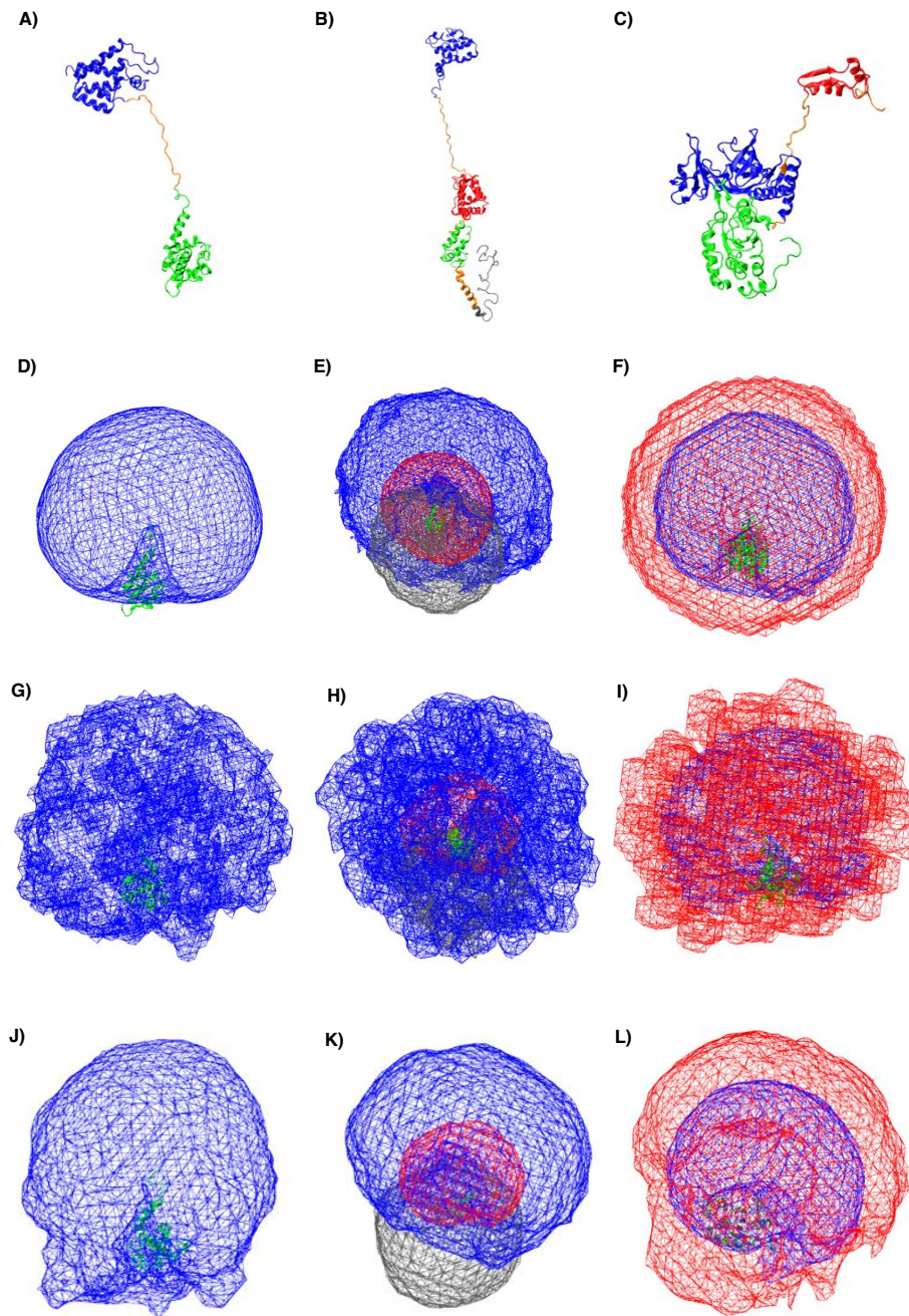
Figure 1: Cartoon representation of A-B system, HIV-1 Gag protein and TraI protein (A-C), and their density plots of conformational coverage from MC simulation (D-F), from subsampled representative structures (G-I) and after TAMD simulations (J-K). A), D), G) and J) A-B system, MA domain is shown in green, NTD domain is shown in blue; B), E), H) and K) the full-length HIV-1 Gag protein the MA 9 domain is shown in blue, the NTD domain is shown in red, the CTD domain is shown in green and the NC domain is shown in grey. B), E) and H) full-length HIV-1 Gag protein is aligned with CTD domain. C), F), I) and L) TraI protein, the first globular domain (residues 381 to 573) is shown in green, the second globular domain (residues 577 to 789) is shown in blue and the third globular domain (residues 804 to 849) is shown in red.
