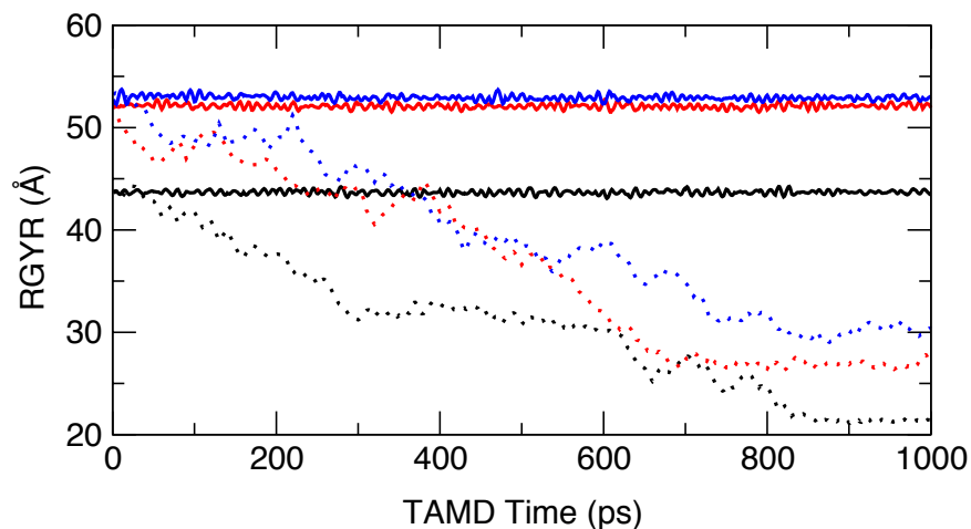
Figure 6: Radii of gyration of A-B system from three representative TAMD simulations with (solid lines) or without (dashed lines) RGYR restraints.
