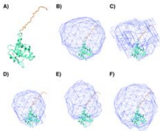
Figure 7: A-tail system and the density plot of different ensembles. A. Cartoon rendering of the A-tail system, extracted from the HIV-GAG protein (residue 1 to 143), tail region is flexible in the simulations and is shown in orange. B. Density plot of the Monte Carlo ensemble. C. Density plot of the sub-sampled ensemble. D. Density plot of the TAMD ensemble without constraints. E. Density plot of the TAMD ensemble with RGYR constraints imposed on the entire A-tail system. F. Density plot of the TAMD ensemble with RGYR constraints imposed on the tail only.
