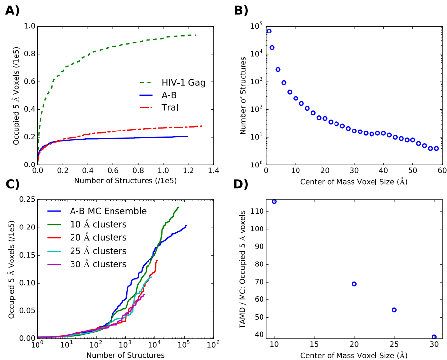
Figure 2: Representative characteristics of subsampling MC ensembles. A) The total number of unique 5 Å voxels occupied by an alpha carbon as a function of the number of structures in each MC ensemble. B) The number of center of mass voxels occupied by structures in the A-B MC Ensemble as a function of voxel size. C) Comparison between the total number of unique 5 Å voxels occupied by an alpha carbon for the A-B MC Ensemble and the ensembles created using TAMD simulations on various sizes center of mass voxels. D) TAMD/MC ratio of the total number of unique 5 Å voxels occupied by an alpha carbon as a function of the center of mass voxel size.
