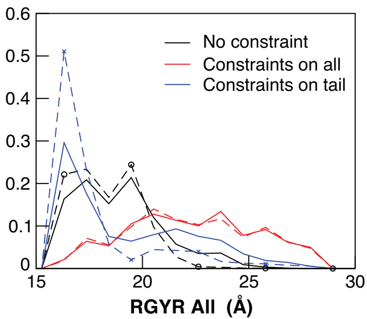
Figure 9: A). RGYR distribution of the A-tail system from TAMD simulations. Solid lines indicate the distribution from the first 500ps simulations and dashed lines indicate the distribution from the last 500ps simulations.
