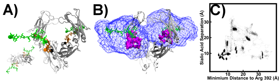
Figure 12: TAMd simulation of the N-glycan in the PTerm455 construct based on IgA1. (A) The location of the N-linked glycans in the Fc fragment of the construct for both the crystal structure (orange) and the initial structure used for simulation which is based on the model of Boehm et al. [40] (green). The C1 atoms of the terminal sialic acid monosaccharides are shown as spheres. The carbon alpha of arginine 392 is shown as a black sphere. The inset figure shows the structure viewed along the symmetry axis. (B) Occupancy plot showing the space explored by the N-glycans during simulations. The blue wireframe volume represents all regions of space sampled during the simulation and the red shaded region that sampled by more than 50 % of the simulation frames. The crystal structure glycan conformation (orange) is shown for comparison. (C) The variation in glycan conformation observed in the simulation characterized by the minimum distance between a C1 atom of one of the branch terminal sialic acids to arginine 392 and the separation between the two branches.
