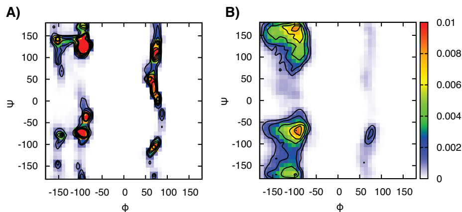
Figure 3: Ramachandran plot for residue 124 in A-B system. A) Dihedral space sampled by 17500 MC configurations generated using only residue 124 as the flexible torsion. B) Dihedral space sampled by MC combined with TAMD simulations. 175 representative configurations were subsampled from 136281 MC configurations and used to carry out independent 1 ns of TAMD simulations. A total of 17500 structures were used in calculating Ramachandran plot shown in B.
