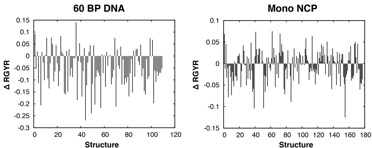
Figure 11: The change of RGyr of the DNA molecules during the TAMd simulations.
