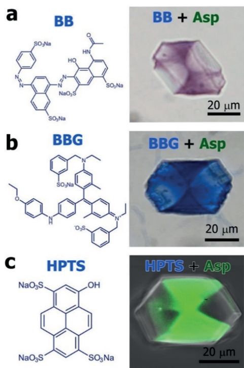
Figure 2. Calcium carbonate crystals precipitated in the presence of Asp and Brilliant Black (BB), Brilliant Blue G (BBG) or 8-hydroxyppyrene-1,3,6-trisulfonic acid (HPTS), under conditions of [Ca^{2+}]:[asp]:[BB] = 250:25:0.5 and [Ca^{2+}]:[asp]:[BBG, HPTS] = 250:25:1 . Non-uniform occlusion is seen.
