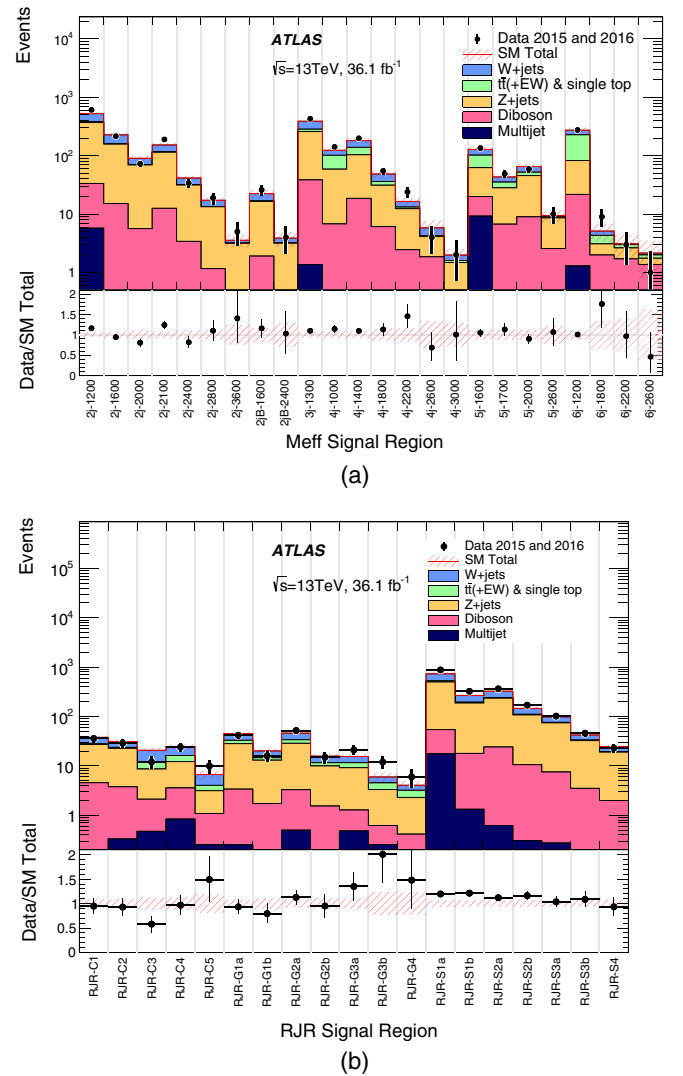
FIG. 12. Comparison of the observed and expected event yields as a function of signal region in the (a) Meff-based and (b) RJR-based searches. The background predictions are those obtained from the background-only fits, presented in Tables V and VI. The bottom graph shows the ratio of observed data yields to the total predicted background. The hatched (red) error bands indicate the combined experimental and MC statistical uncertainties.
