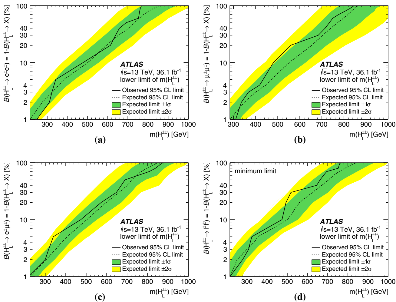
Fig. 13 Lower limit on the H_L^{\pm\pm} boson mass as a function of the branching ratio B(H_L^{\pm\pm} \rightarrow \ell^\pm \ell^\pm) . Several cases are presented: a H_L^{\pm\pm} decays only into electrons and “X”, b H_L^{\pm\pm} decays only into muons and
