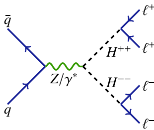
Fig. 1 Feynman diagram of the pair production process pp \rightarrow H^{++} H^{--} . The analysis studies only the electron and muon channels, where at least one of the lepton pairs is e^\pm e^\pm , e^\pm \mu^\pm , or \mu^\pm \mu^\pm
