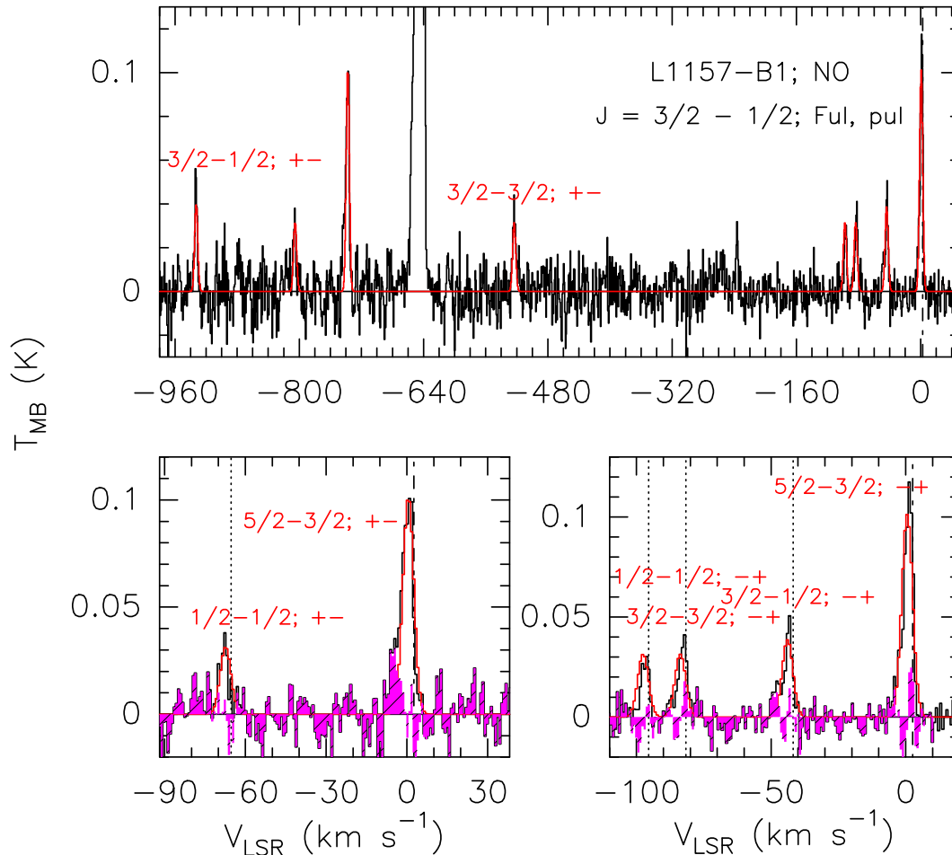
Figure 6. Upper panel: emission due to the NO {}^2\Pi_{1/2} J = 3/2-1/2 spectral pattern (black histogram; see Table 1; in T_{\text{mb}} scale after correction for beam dilution, see the text) observed towards L1157-B1 with the IRAM 30-m antenna. The red line shows the best fit obtained with the GILDAS-CLASS package using the simultaneous fit of all the hyperfine components (see Table 2). For sake of clarity, the hyperfine components that are not indicated in the upper panel are labelled in the zoom-in in the lower panels. The spectrum is centred at the frequency of the hyperfine component F_{\text{ul}} = 5/2-3/2; p_{\text{ul}} = - \rightarrow + (150 176.48 MHz). The vertical dashed line indicates the ambient LSR velocity ( +2.6 \text{ km s}^{-1} ; Bachiller et al. 2001). Bottom-right panel: zoom-in of the upper panel. Dotted lines point the hyperfine components falling in that portion of the spectrum. The purple filled histogram shows the residual after Gaussian fit (red) of the NO emission (black). Bottom-left panel: zoom-in of the upper panel, after having centred the spectrum at the frequency of the hyperfine component F_{\text{ul}} = 5/2-3/2; p_{\text{ul}} = + \rightarrow - (150 546.52 MHz).
