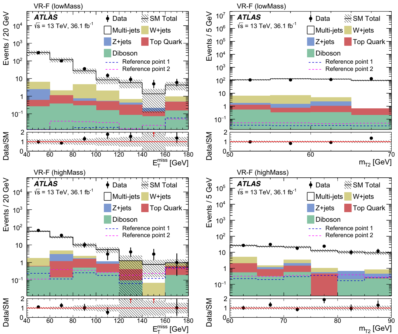
Fig. 3 The E_T^{\text{miss}} (left) and m_{T2} (right) distributions in the multi-jet background VR-F for SR-lowMass (top) and VR-F for SR-highMass (bottom). The stacked histograms show the contribution of the non-multi-jet SM backgrounds from MC simulation. The multi-jet contribution is estimated from data using the ABCD method. The hatched
