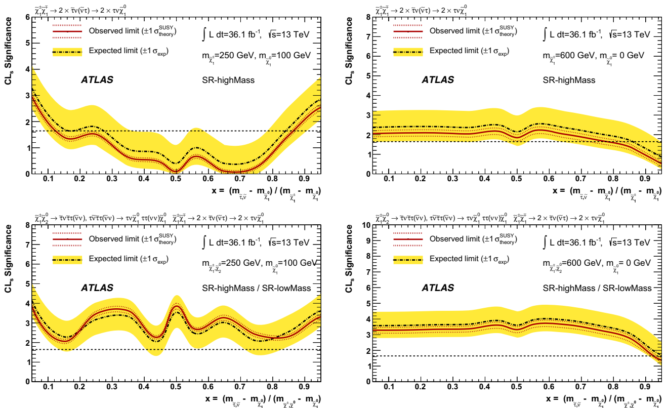
Fig. 8 The CL_s significance for the benchmark models described in Sect. 3 as a function of the parameter x . The benchmark scenario with large mass splitting ( m(\tilde{\chi}_1^\pm, \tilde{\chi}_2^0) = 600 GeV and m(\tilde{\chi}_1^0) = 0 GeV) is shown on the right, and the compressed benchmark scenario ( m(\tilde{\chi}_1^\pm, \tilde{\chi}_2^0) = 250 GeV and m(\tilde{\chi}_1^0) = 100 GeV) on the left, for
