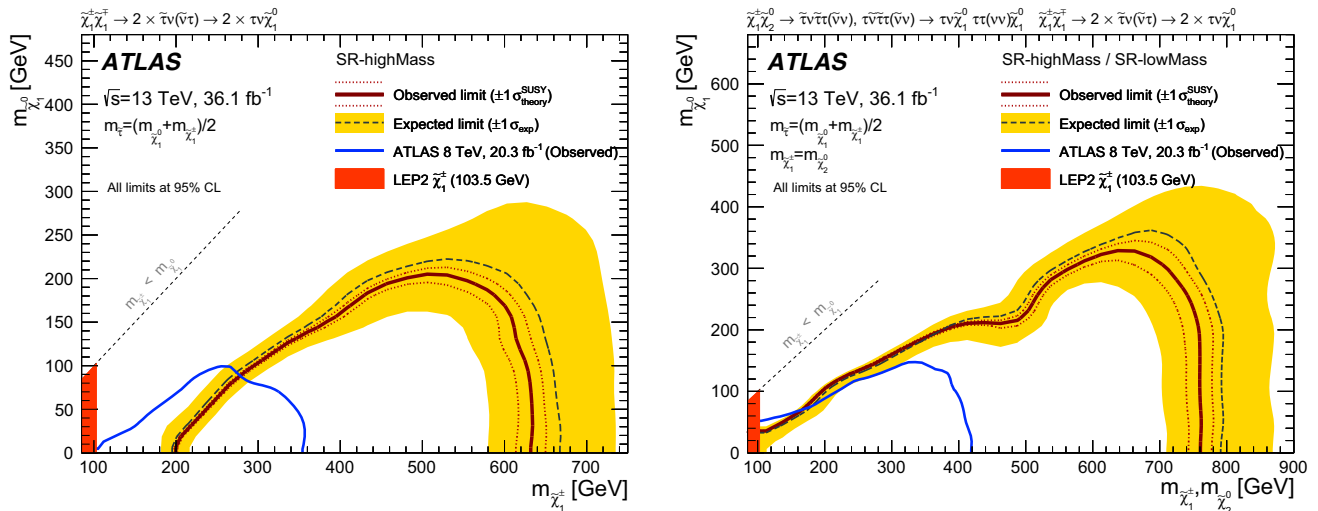
Fig. 7 The 95% CL exclusion contours for simplified models with \tilde{\chi}_1^+ \tilde{\chi}_1^- production (left) and production of \tilde{\chi}_1^+ \tilde{\chi}_1^- and \tilde{\chi}_1^\pm \tilde{\chi}_2^0 (right). The text provides details of exclusion curves and uncertainty bands.
