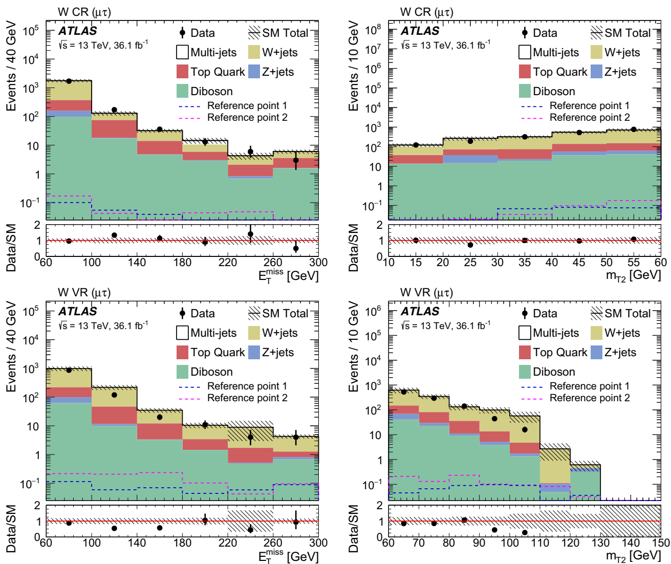
Fig. 4 The E_T^{\text{miss}} (left) and m_{T2} (right) distributions in the W -CR (top) and W -VR (bottom) regions. The SM backgrounds other than multi-jet production are estimated from MC simulation. The contribution of W +jets events is scaled to the fit result. The multi-jet contribution is estimated from data using the OS - SS method. The hatched bands represent
