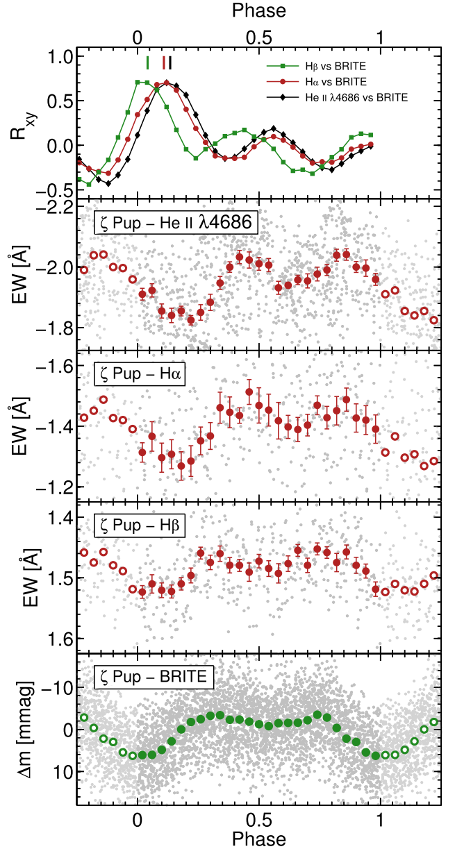
Figure 18. First four panels from bottom to top: light variations of \zeta Pup as observed by BRITE phased with the stellar rotation period, along with the phased time series of EWs of the H \beta , H \alpha and He II \lambda 4686 line profiles of the star. The vertical scale on the panel for H \beta is exactly twice larger than the vertical scales on He II \lambda 4686 and H \alpha . Upper panel: cross-correlation sequences of the EW variations with respect to the light variations observed by BRITE . The measured phase delays extracted through Gaussian fits to the first main cross-correlation peaks are indicated by the vertical markers (the Gaussian fits themselves are not overplotted for the sake of visibility).
