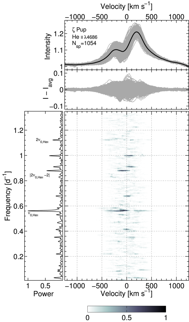
Figure 14. Global time series analysis of the He II 4686 wind emission-line profile of \zeta Pup. Top: the 1054 profiles of the line as recorded throughout the entire campaign (grey) along with their average (black). Middle: difference profiles with respect to the average profile. Main: CLEAN periodogram per Doppler velocity within \pm 1275 km s ^{-1} for the time series of difference spectra, obtained after 10 CLEAN iterations. The side panel depicts the normalized integrated periodogram power within Doppler velocities \pm 500 km s ^{-1} where most of the LPVs are detected.
