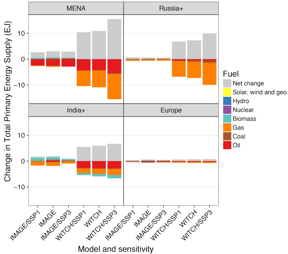
Supplementary Figure 16. Sensitivity of changes in change of supply of different fuels to different SSP assumptions for four representative regions. All changes are shown relative to the relevant SSP Baseline under low oil prices. “Solar, wind and geo.” indicates the aggregate change in solar, wind and geothermal power. Positive values of “Net change” indicate a decrease in the total primary energy supply, negative values an increase. Central scenario is the main scenario from the paper and consistent with SSP2 assumptions (see Supplementary Text 7).
